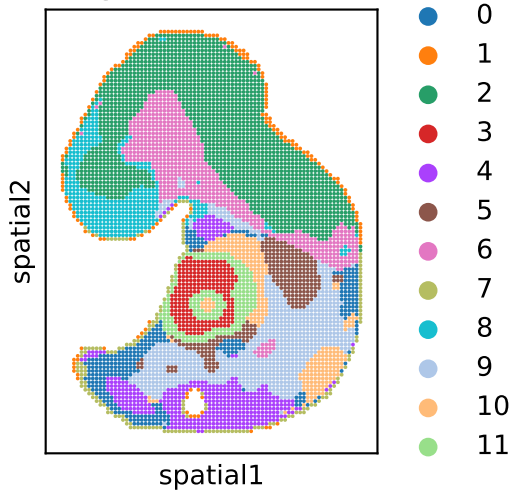
AugGCL (ARI=0.39)
