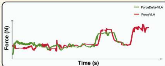
ForceDelta-VLA: Success
