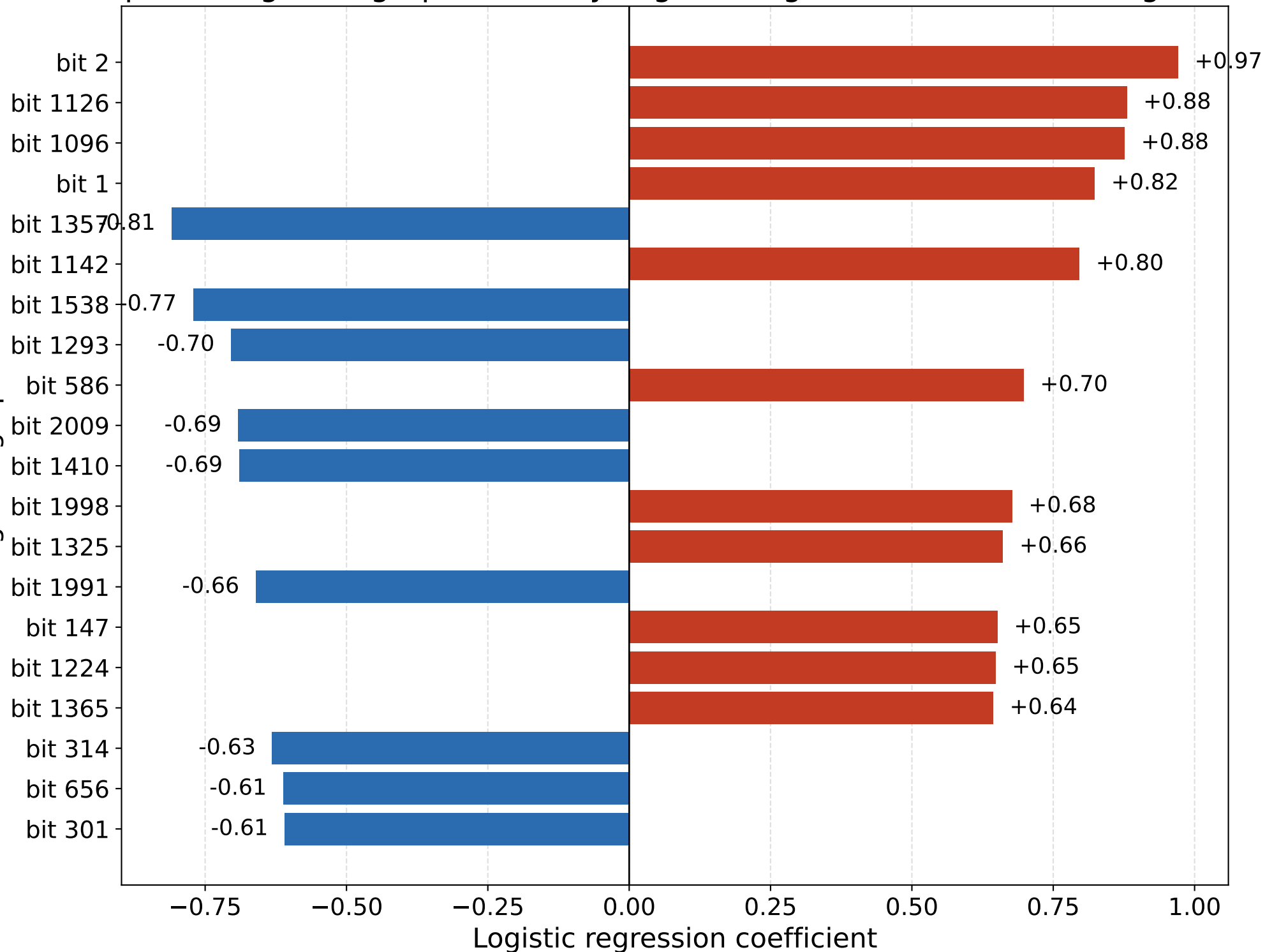
Top 20 Morgan Fingerprint Bits by Logistic Regression Coefficient Magnitude
