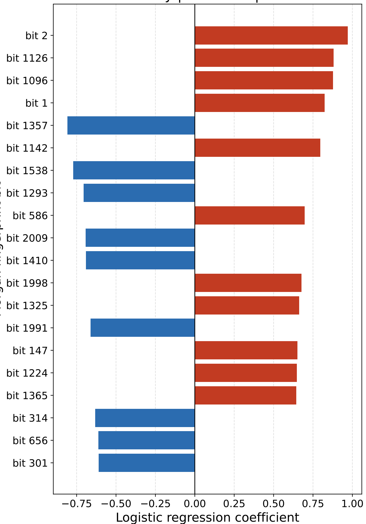
Top 20 Morgan FP bits by |coefficient|
