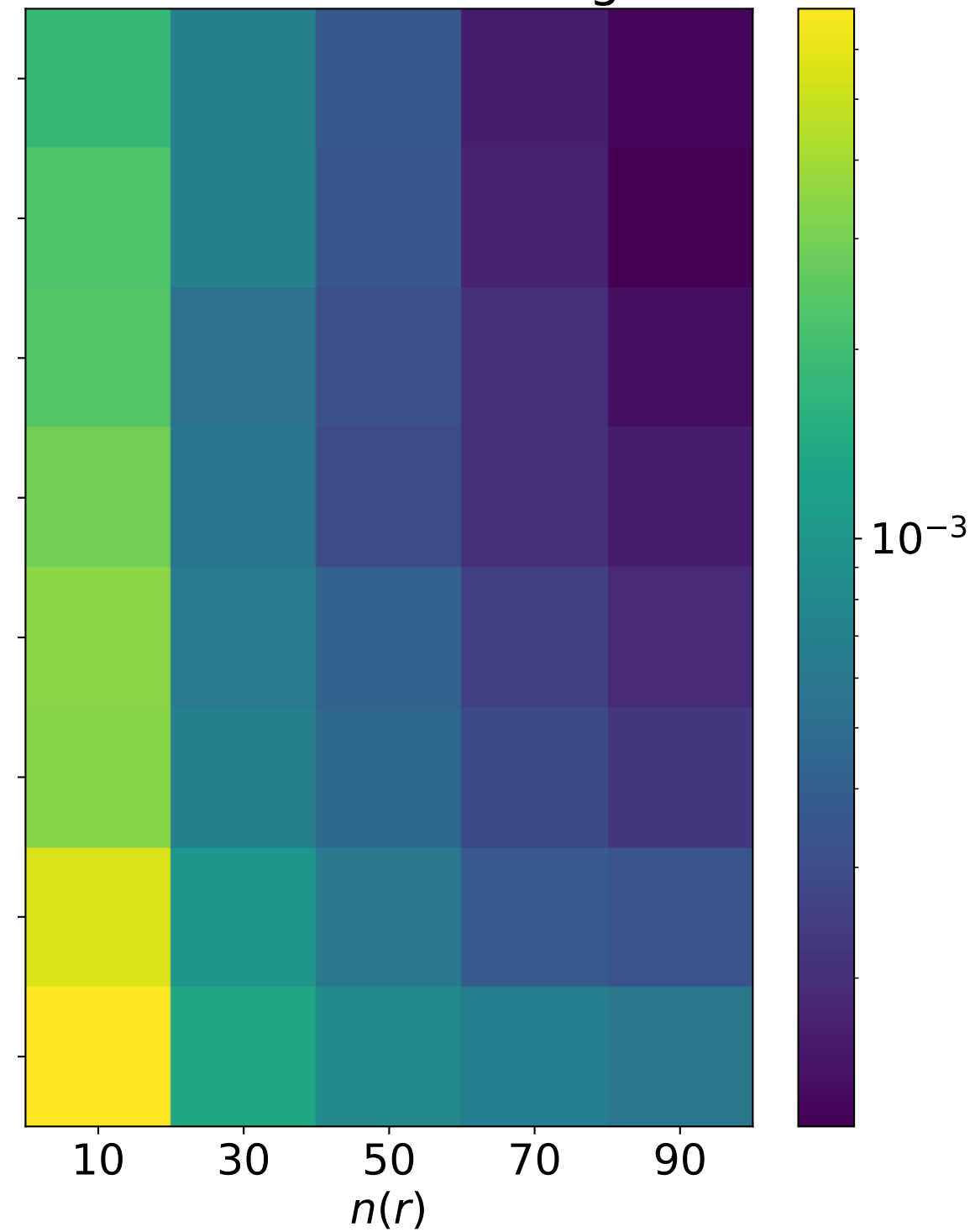
Relative error for integral 1
