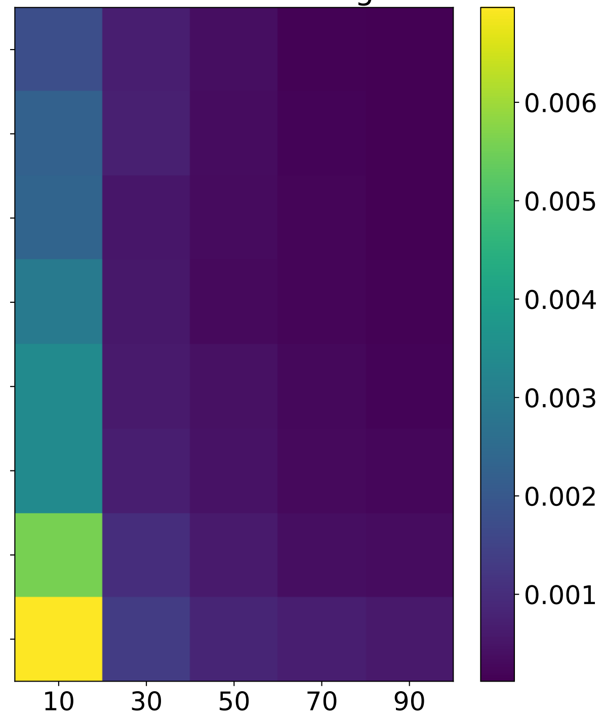
Relative error for integral 1
