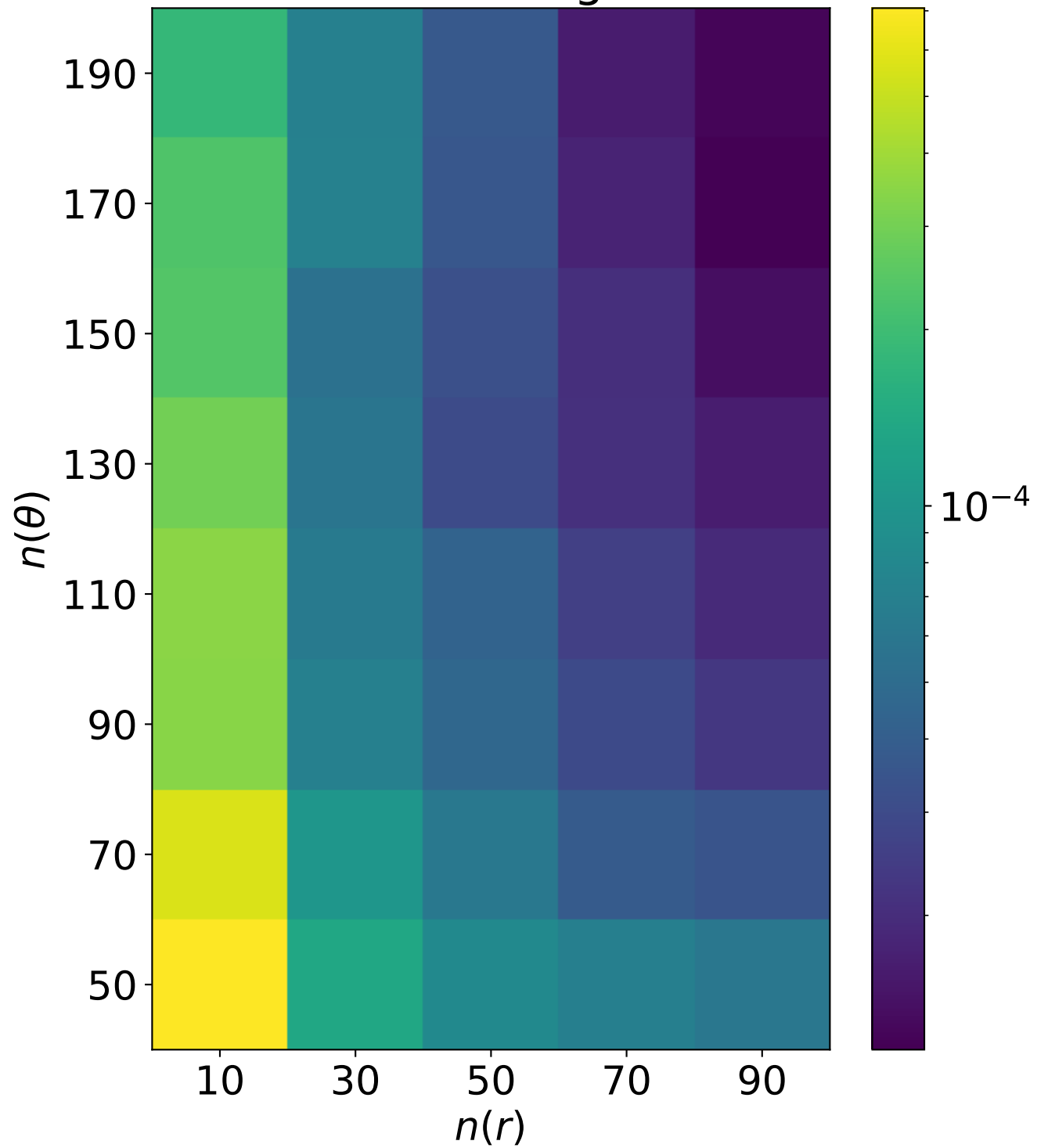
Error for integral 1
