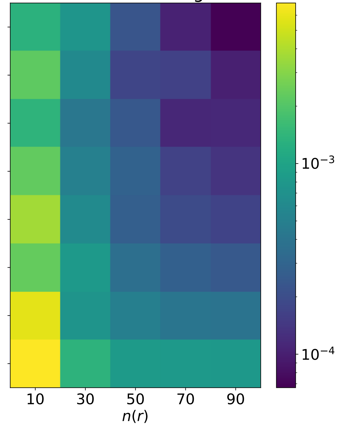
Relative error for integral 766
