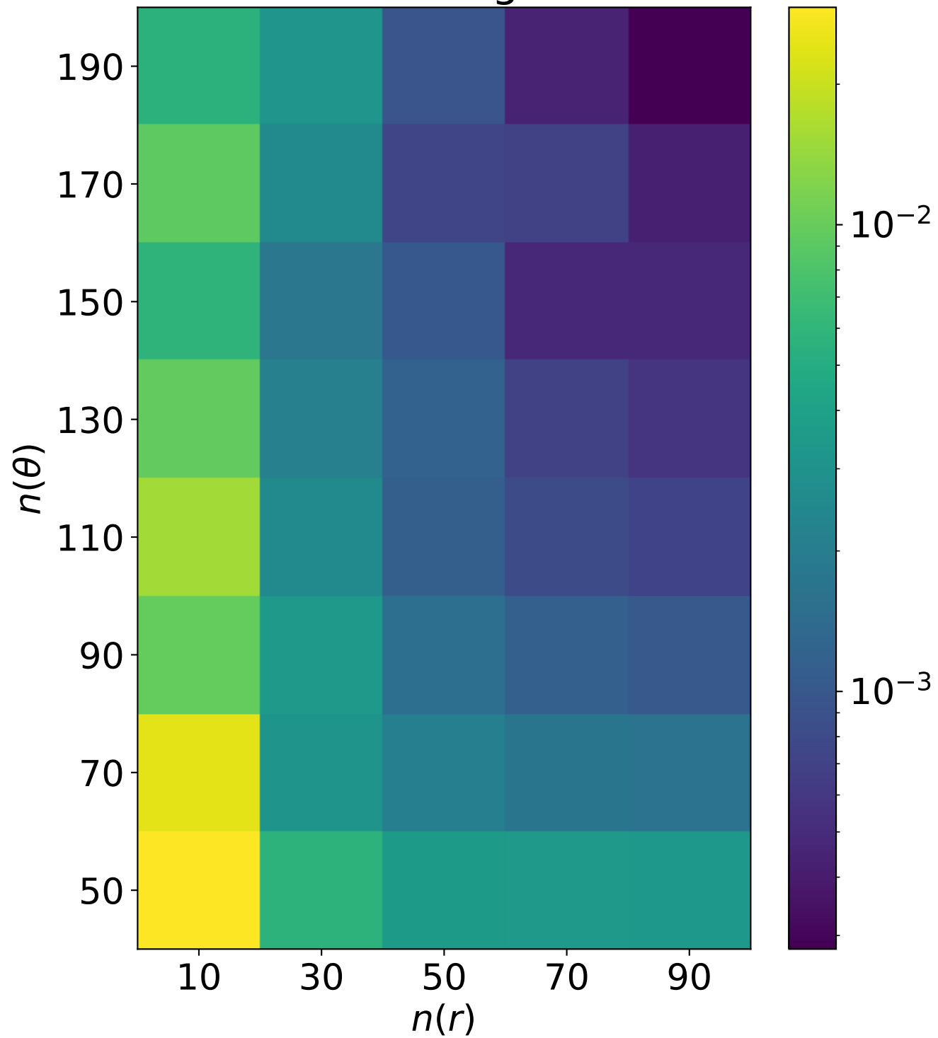
Error for integral 766
