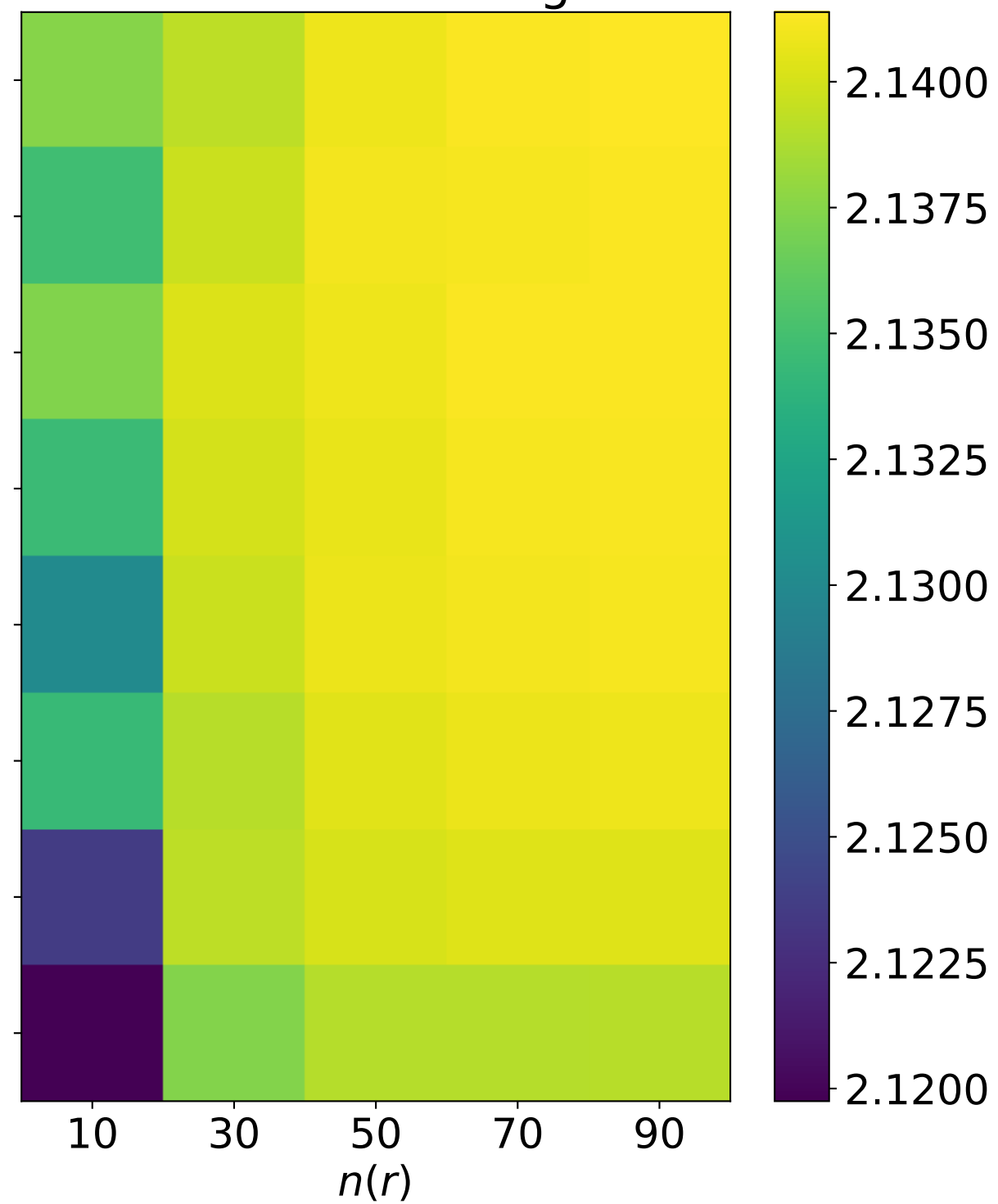
Relative error for integral 766
