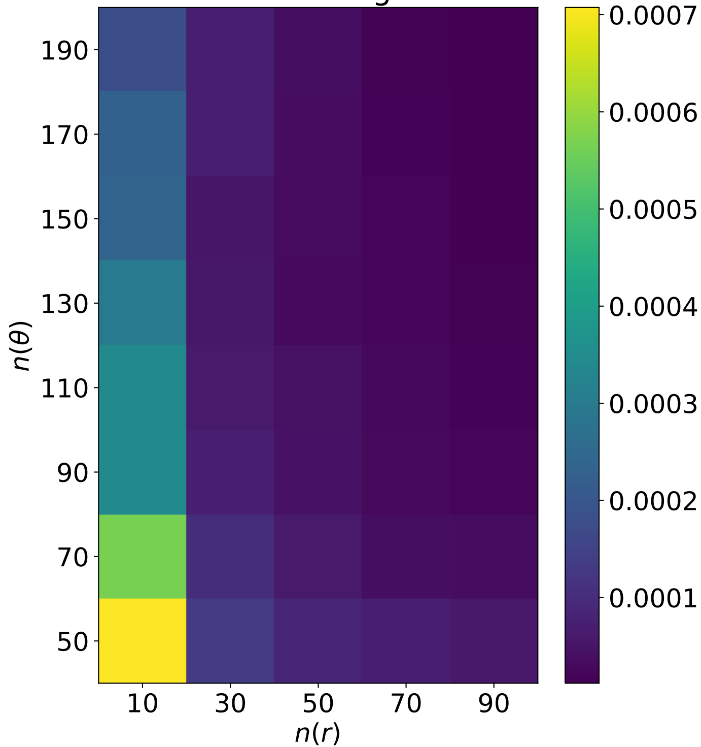
Error for integral 1
