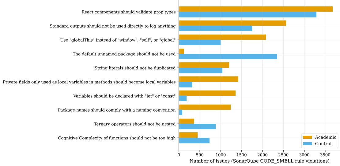
Figure 4: The ten most frequent SonarQube code-smell types, academic vs. control (415 repositories analyzed).
