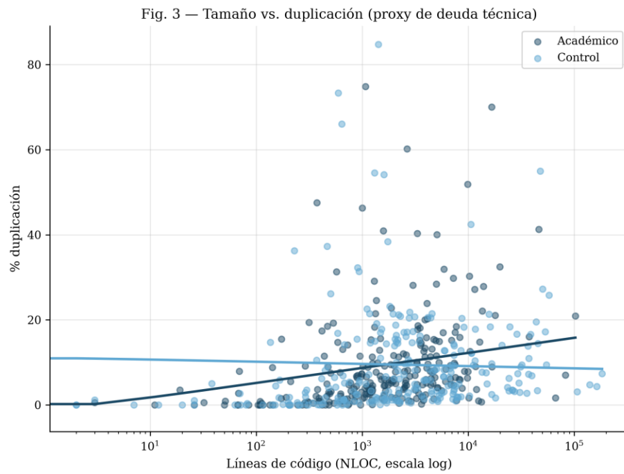
Figure 3. Repository size (lines of code) vs. code duplication, academic vs. control.
