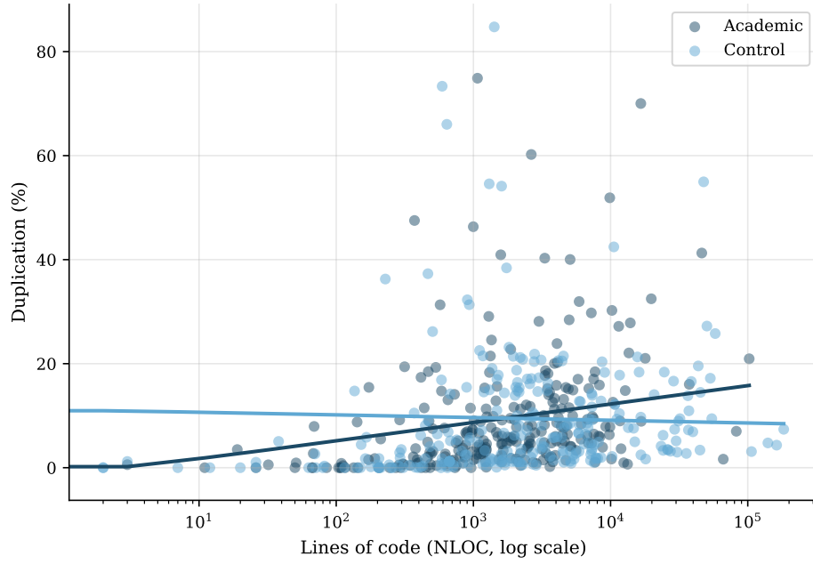
Figure 3: Repository size (lines of code) vs. code duplication, academic vs. control.
