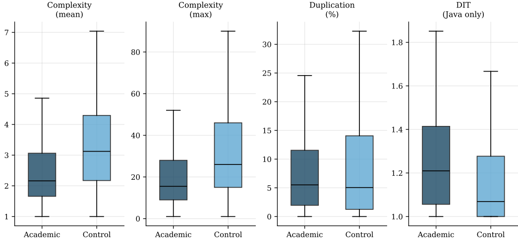
Figure 1: Distribution of key metrics, academic vs. control repositories.
