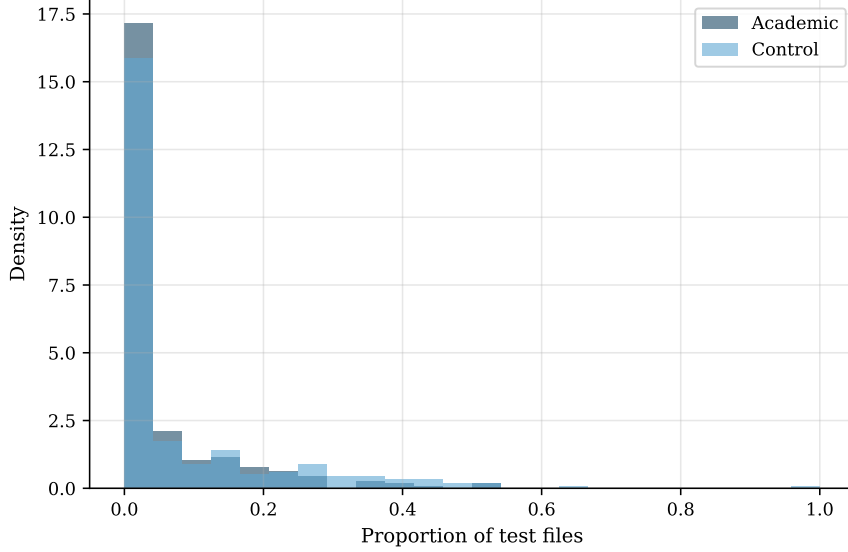
Figure 2: Distribution of the test-file-proportion proxy, academic vs. control.
