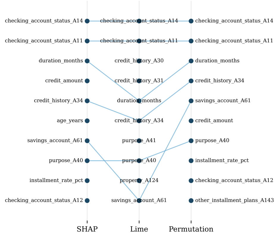
German Credit (Finance)
