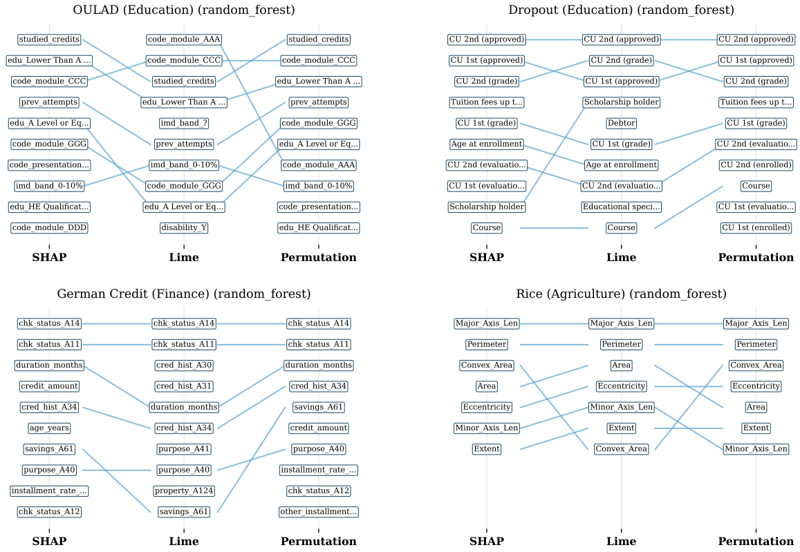
Figure 4: Top-10 features by SHAP, LIME, and permutation importance (random forest), all four datasets; lines connect a feature that appears in the top 10 of both adjacent methods.
