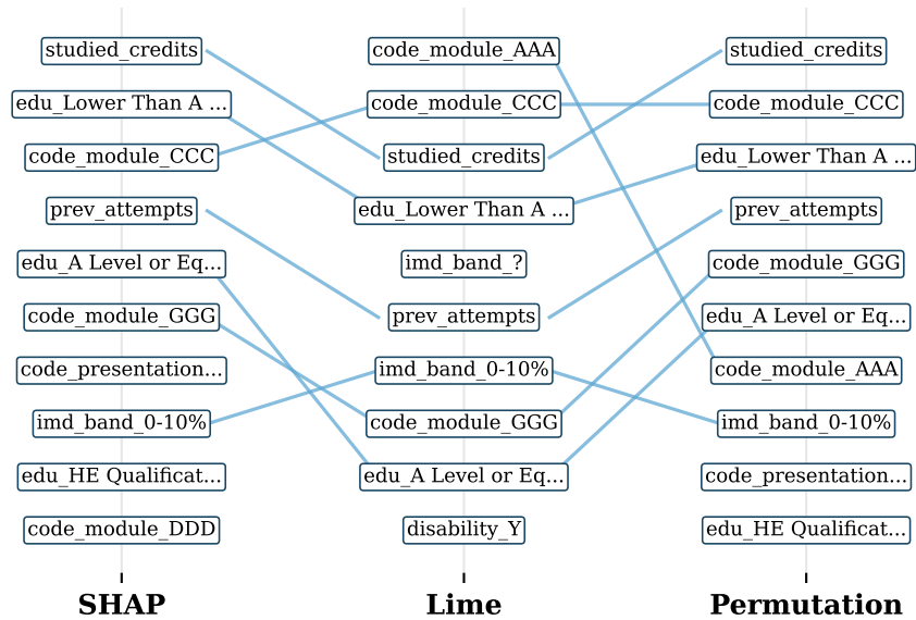
OULAD (Education) (random_forest)
