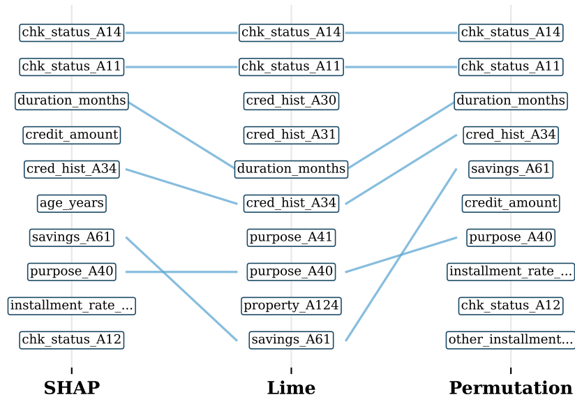
German Credit (Finance) (random_forest)
