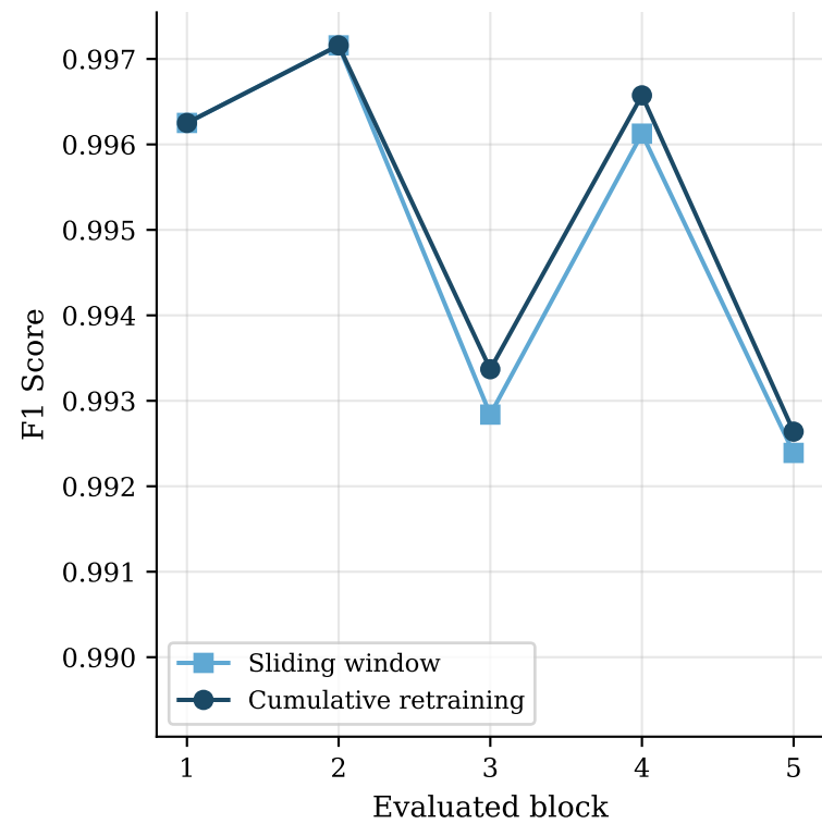
Random Forest
