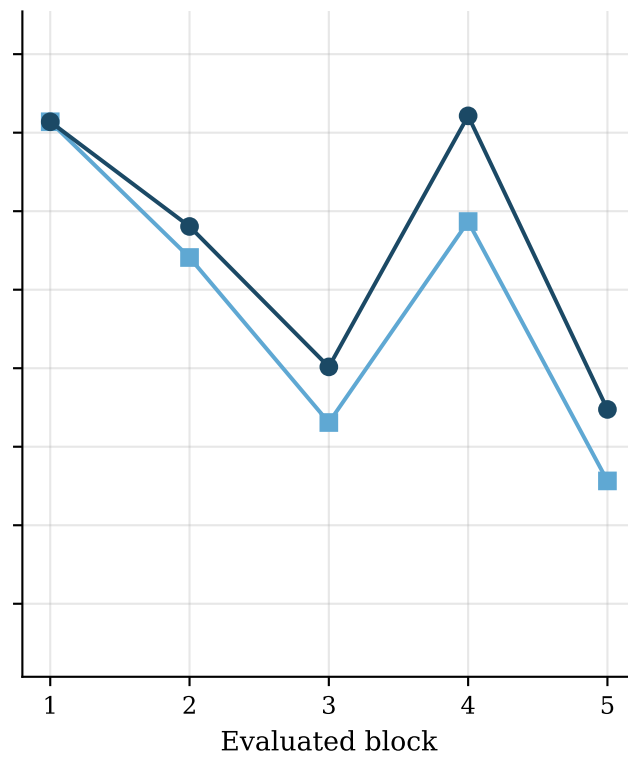
XGBoost
