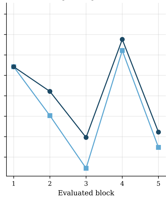
Logistic Regression
