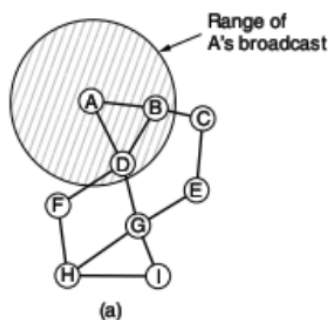
Figure 5-20. (a) Range of A's broadcast.
