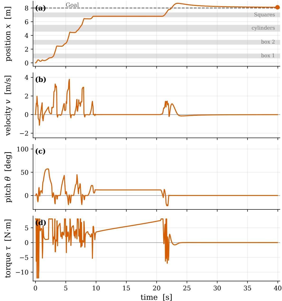
NMPC: Four obstacles until the goal (settle 0.11 m, peak pitch 57°)
