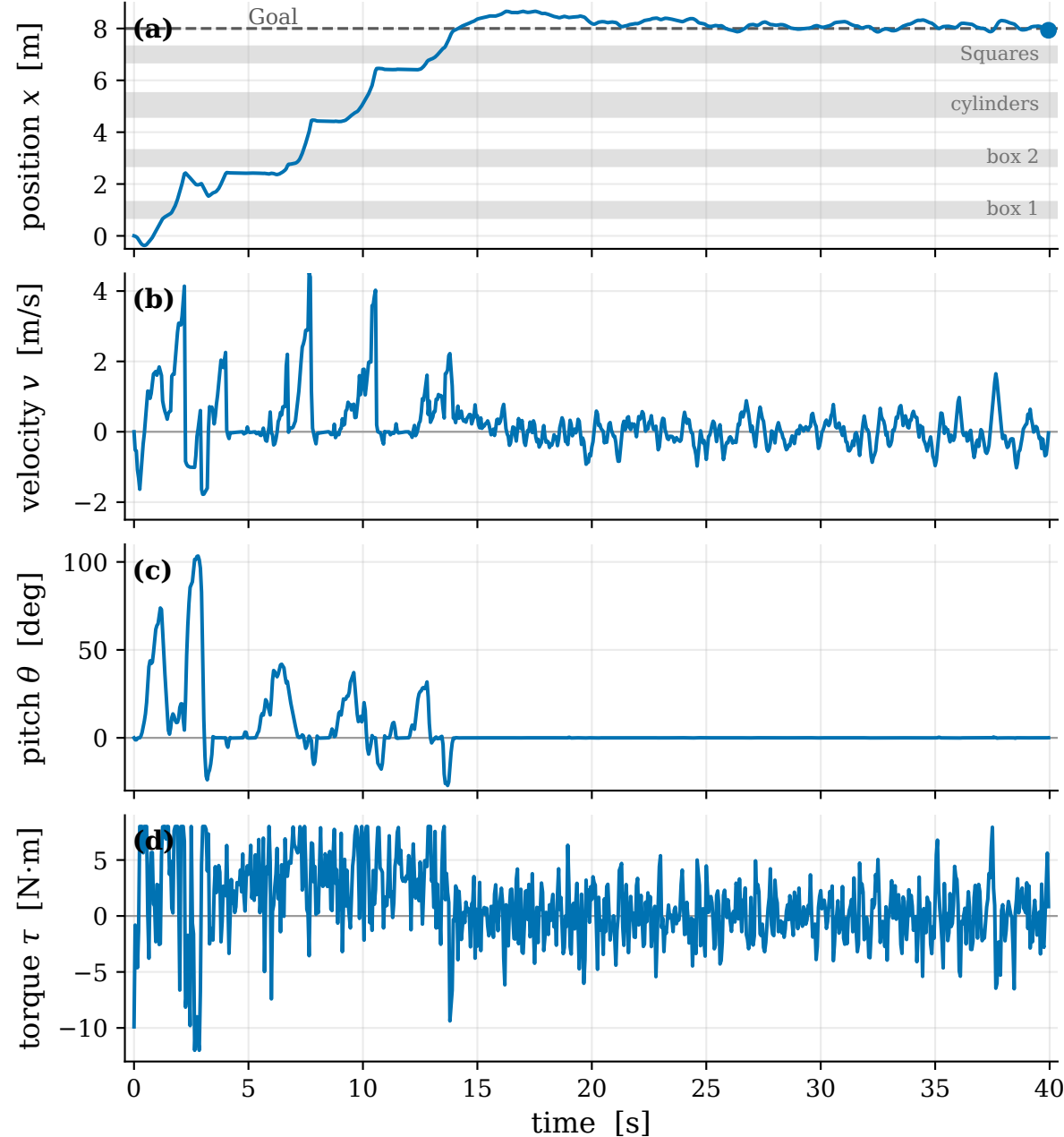
MPPI: Four obstacles until the goal (settle 0.07 m, peak pitch 103°)
