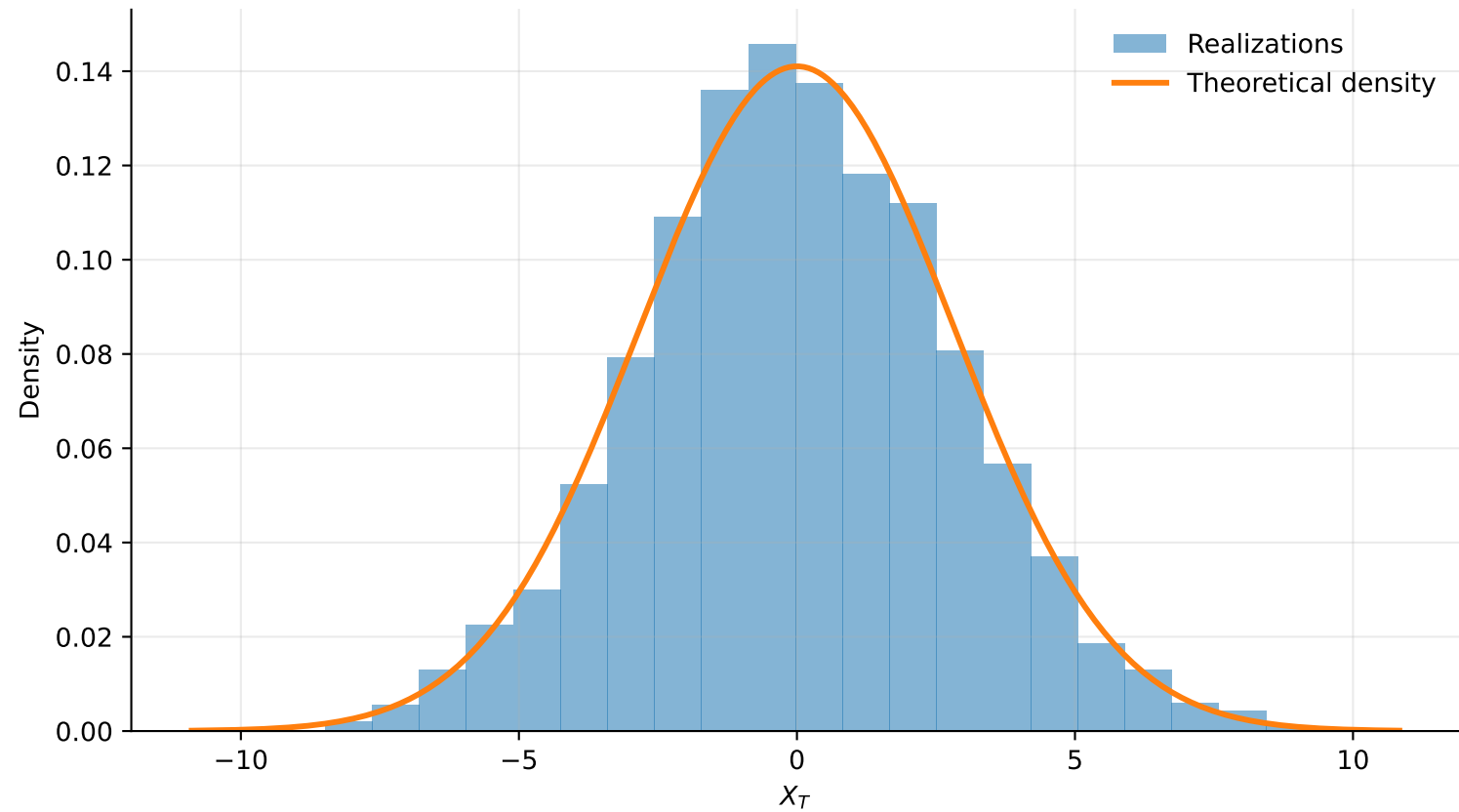
Distribution of X_T for T = 10
