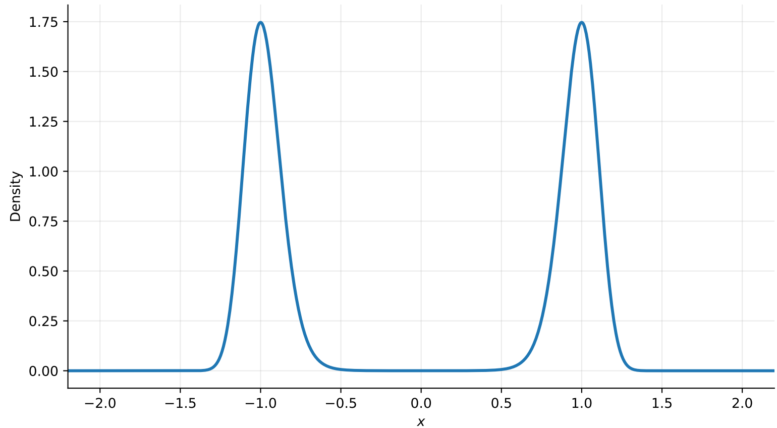
Theoretical Boltzmann Distribution ( D = 0.1 )
