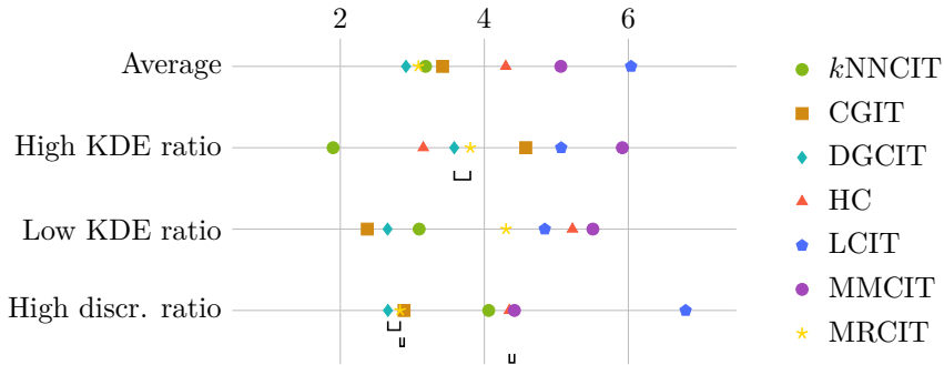
Critical difference diagrams for graph F1-score
