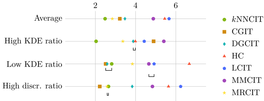
Critical difference diagrams for PDAG SHD-score
