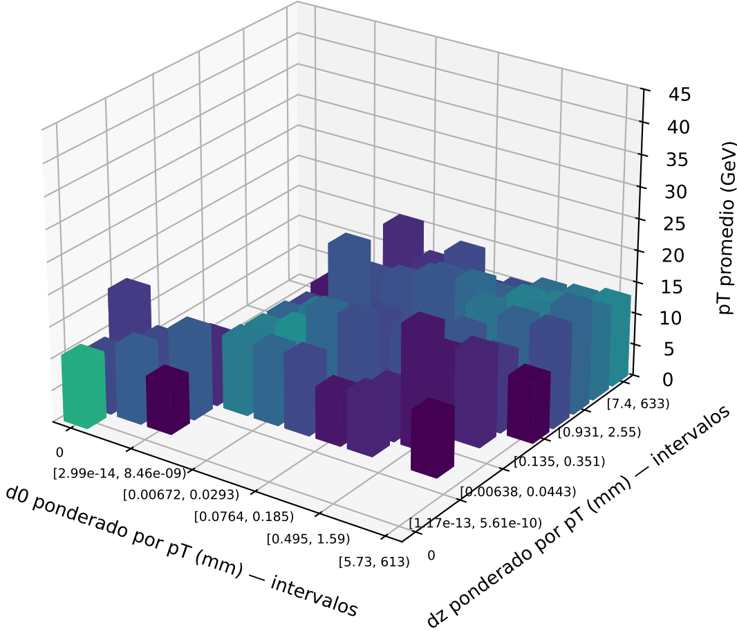
TN — N=57,655
