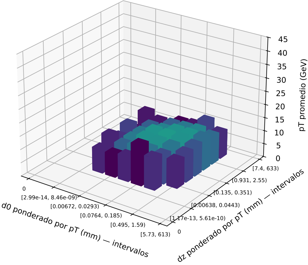
FP — N=2,300
