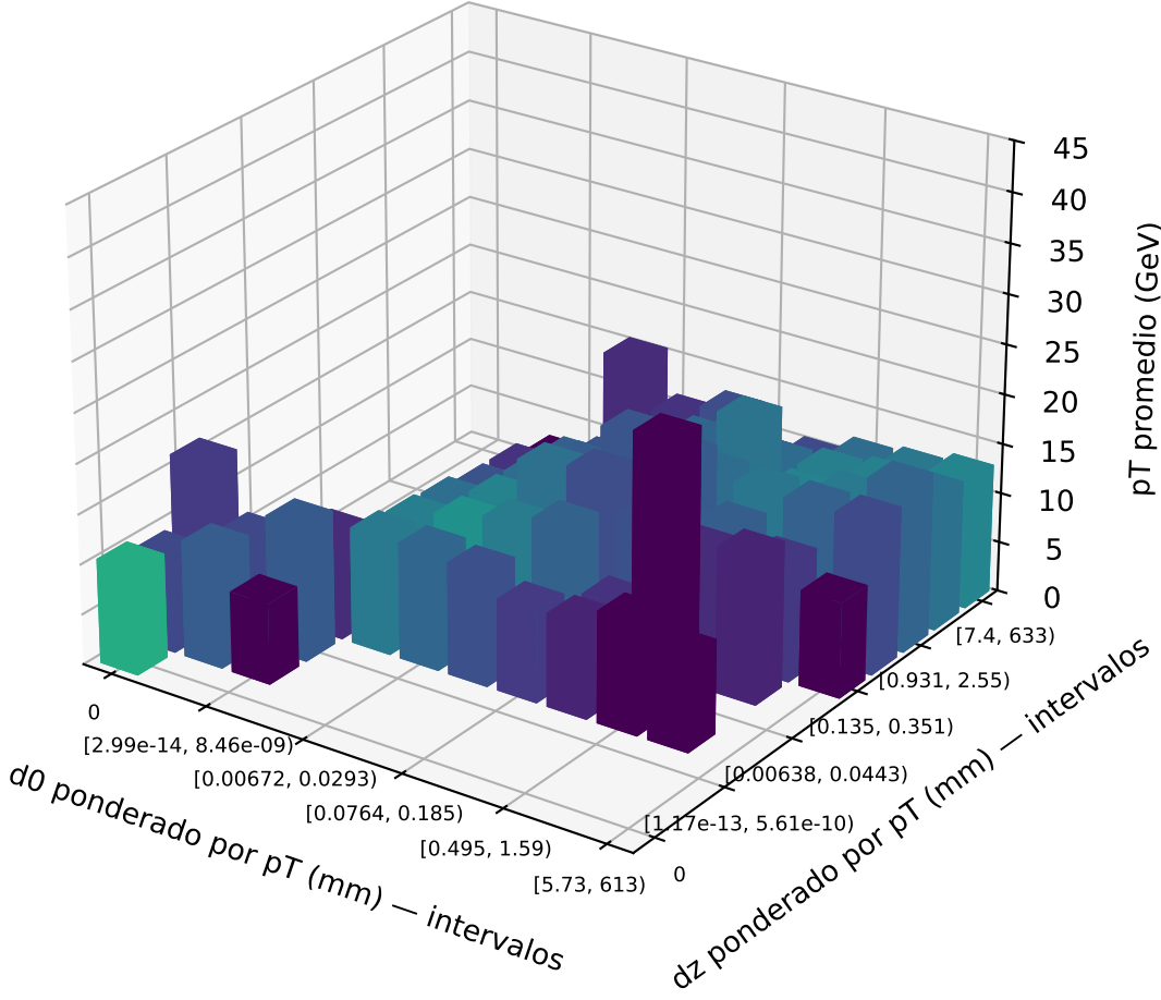
TN — N=58,576
