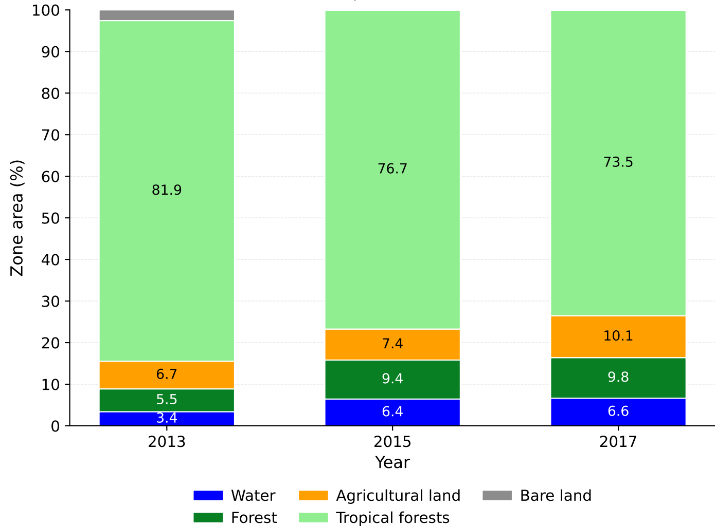
Land-cover composition in runoff zone 1
