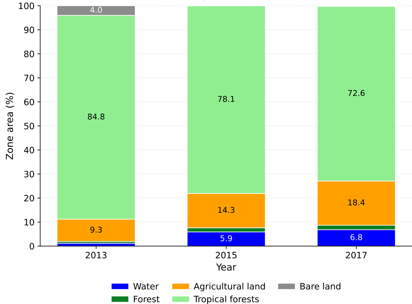
Land-cover composition in runoff zone 5
