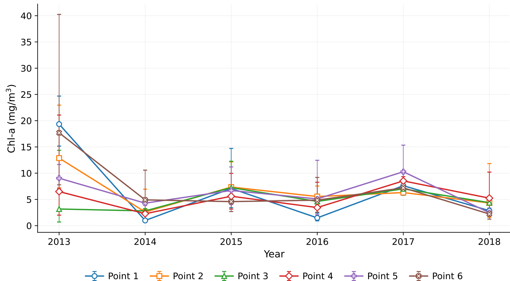
Temporal variation of Cl-a at tributary points
