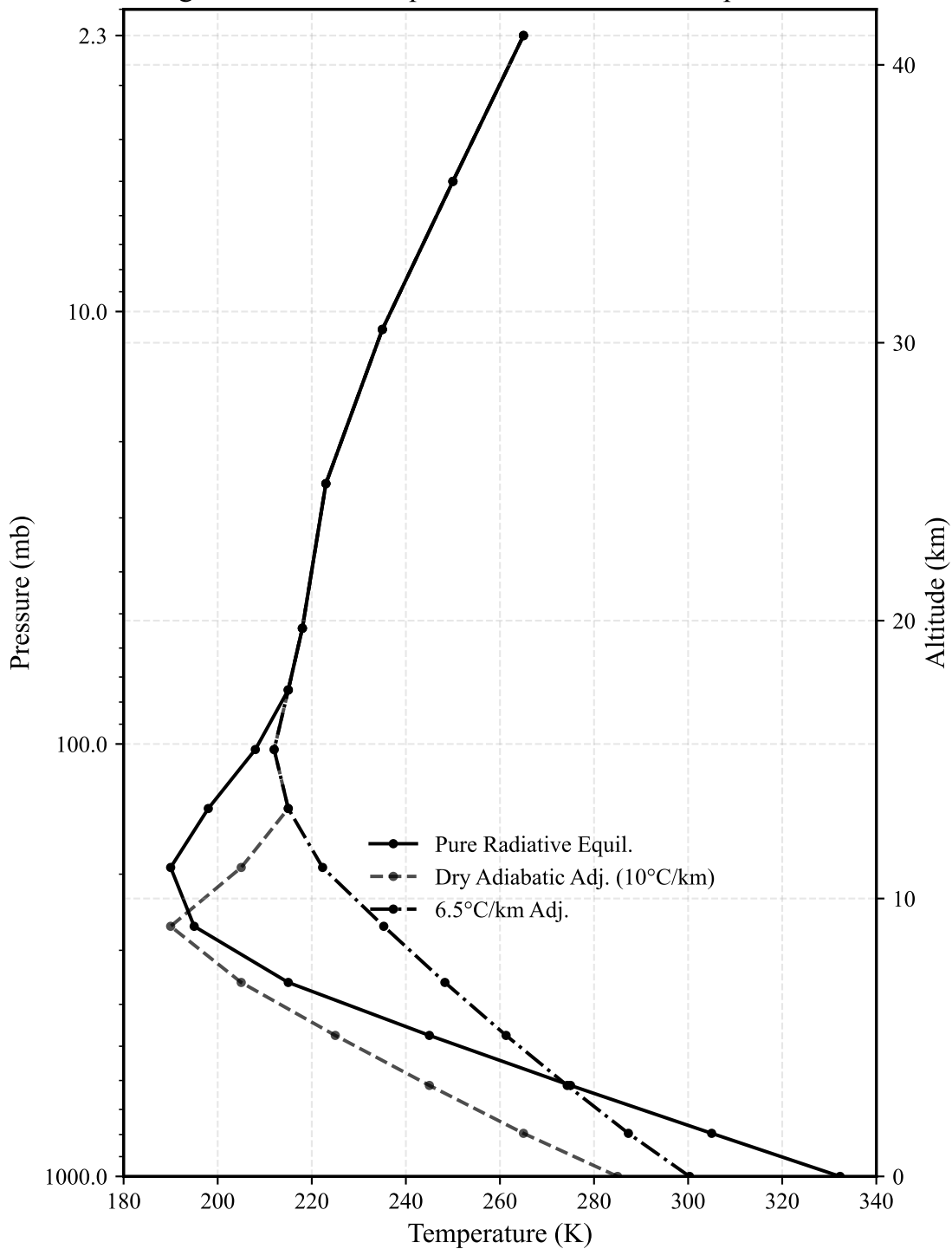
Figure 4: Thermal Equilibrium vs Radiative Equilibrium
