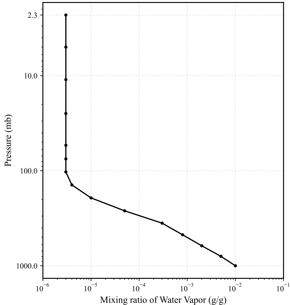
Fig 5a: H_2O Profile (35°N, April)
