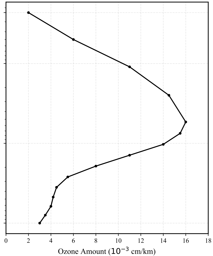
Fig 5b: Ozone Profile (35°N, April)
