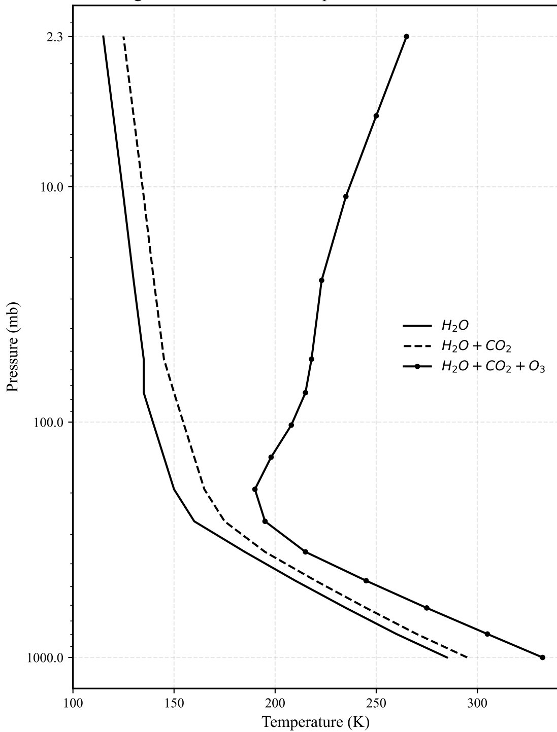
Figure 6a: Pure Radiative Equil. for Various Absorbers
