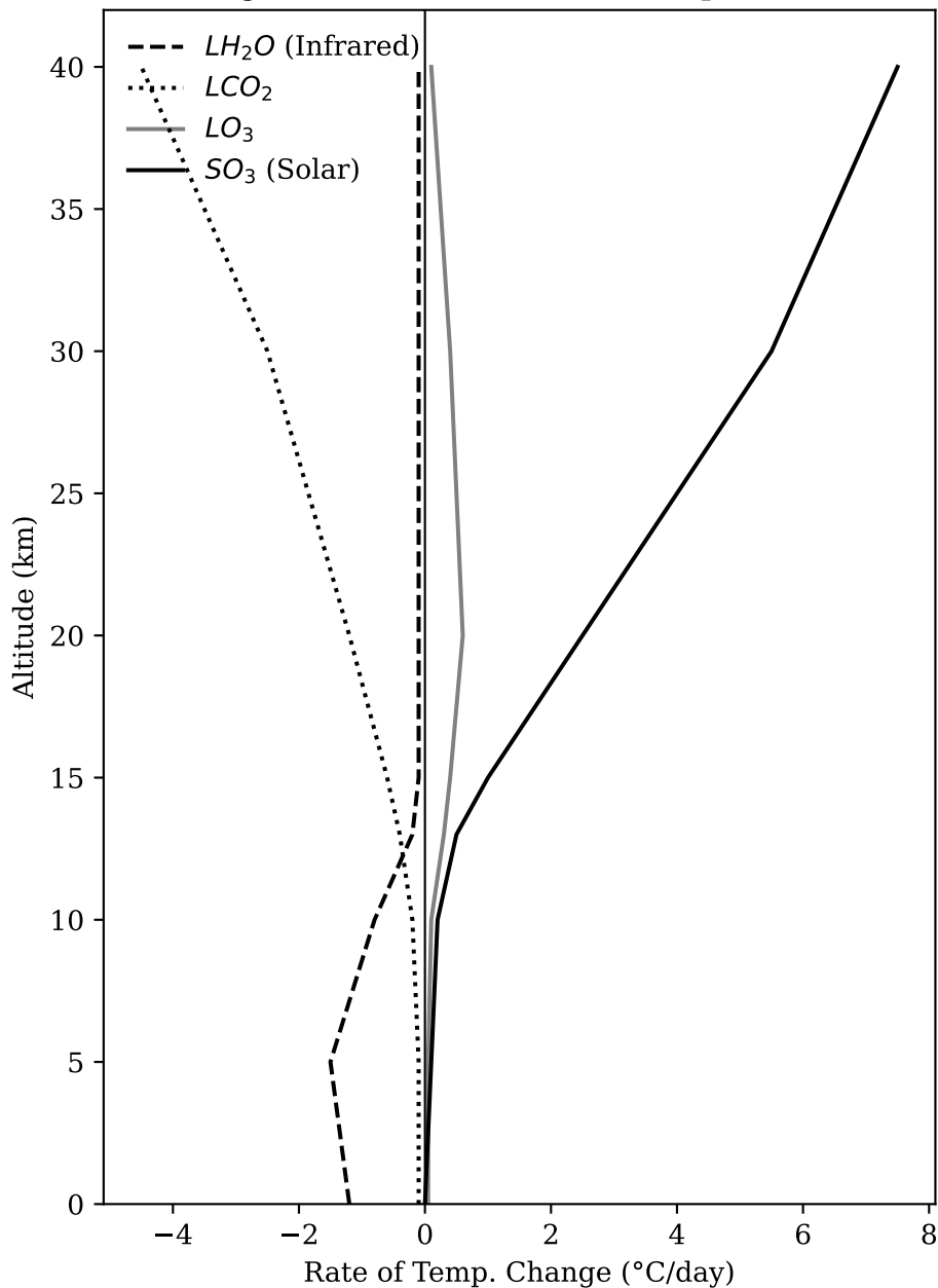
Figure 6b: Heat Balance Components
