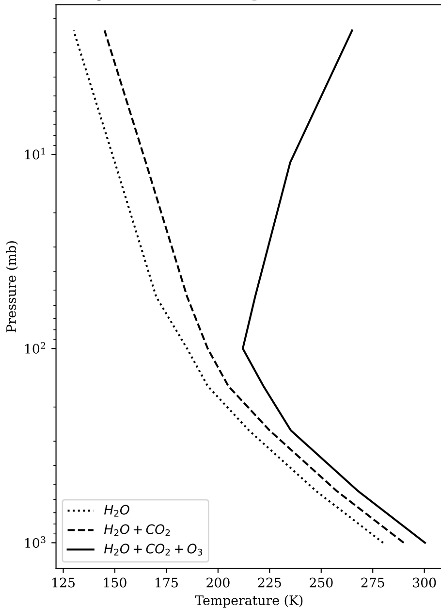
Figure 6c: Thermal Equilibrium (6.5°C/km)
