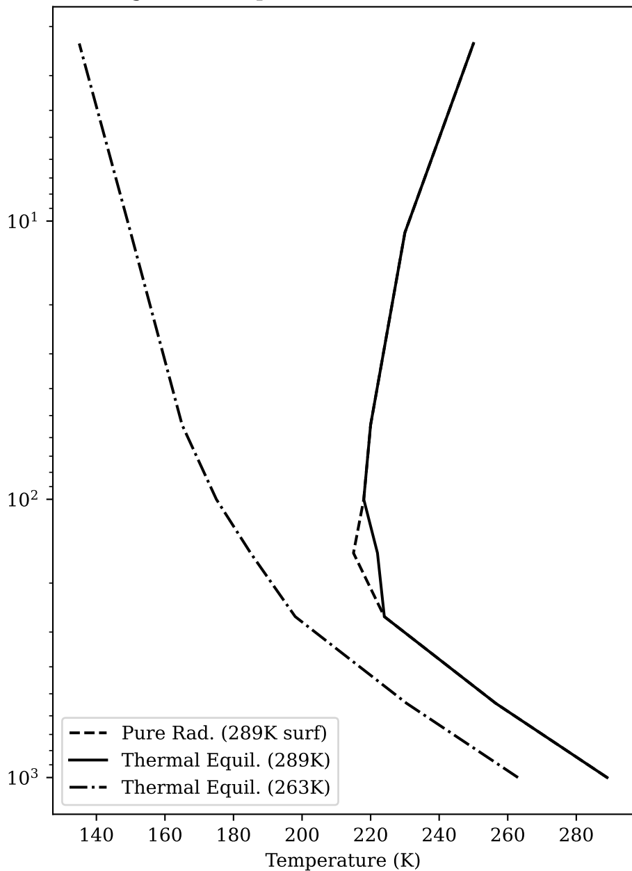
Figure 6d: Equilibrium without Insolation
