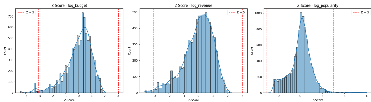
Figura 6: Histogramas Z-Score.
