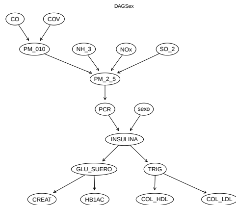
Figure 4: DAG 3 with sex variable
