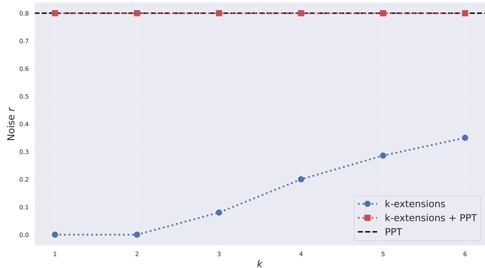
Random Robustness of Entanglement (Werner state p = 0.6 )
