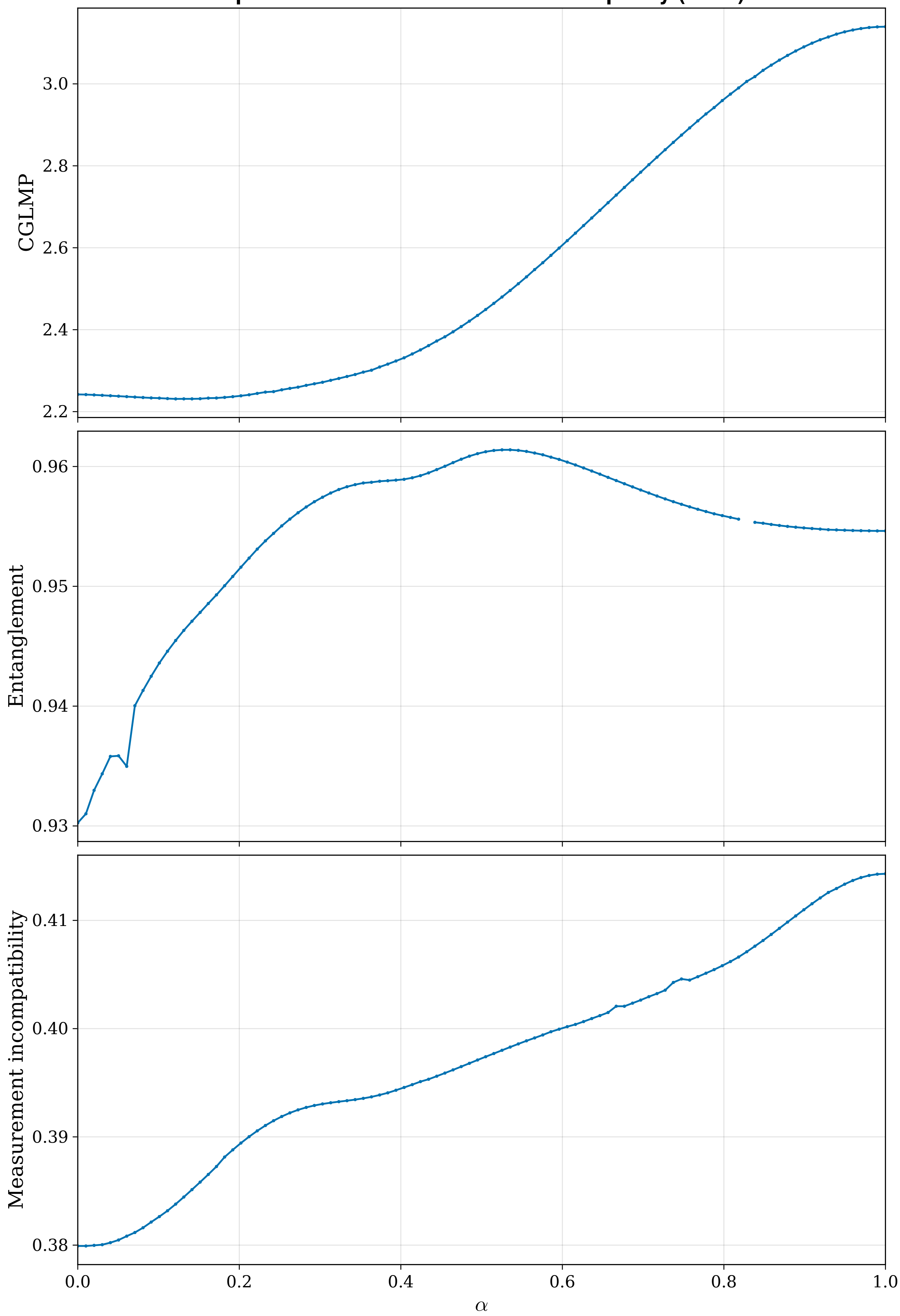
Optimal violation of the CGLMP inequality (d=10)
