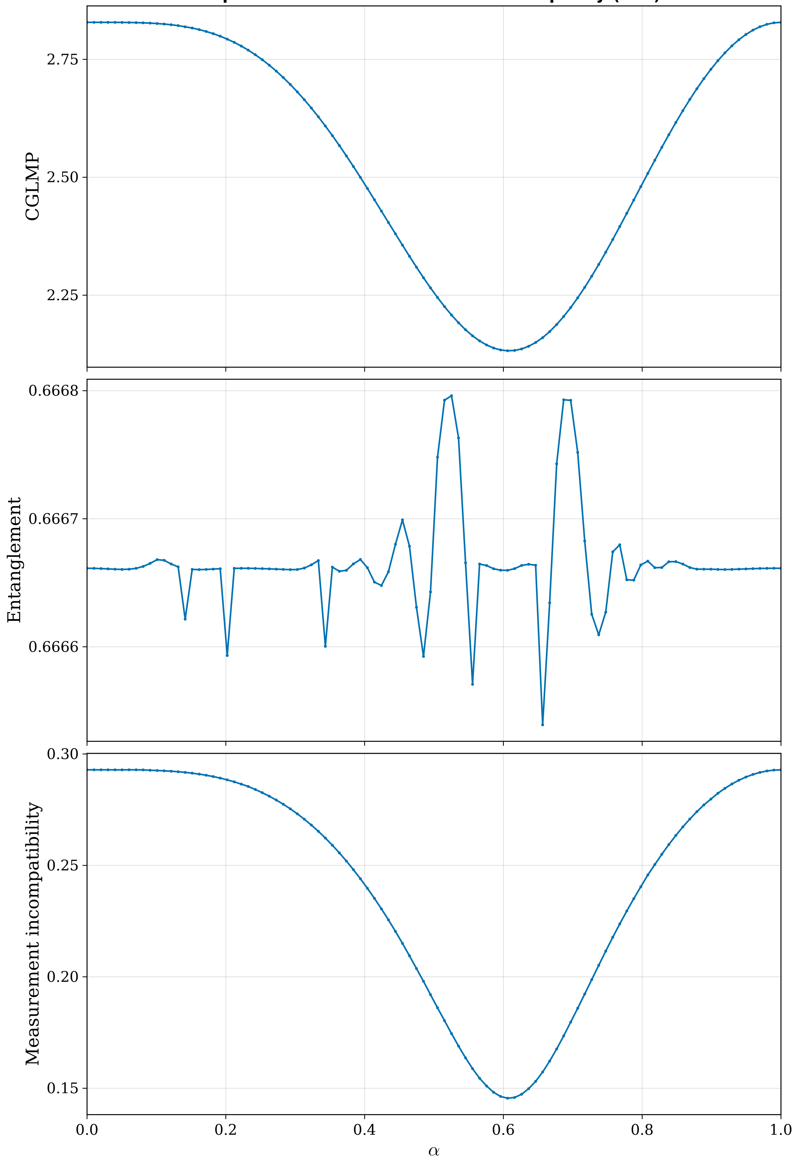
Optimal violation of the CGLMP inequality (d=2)
