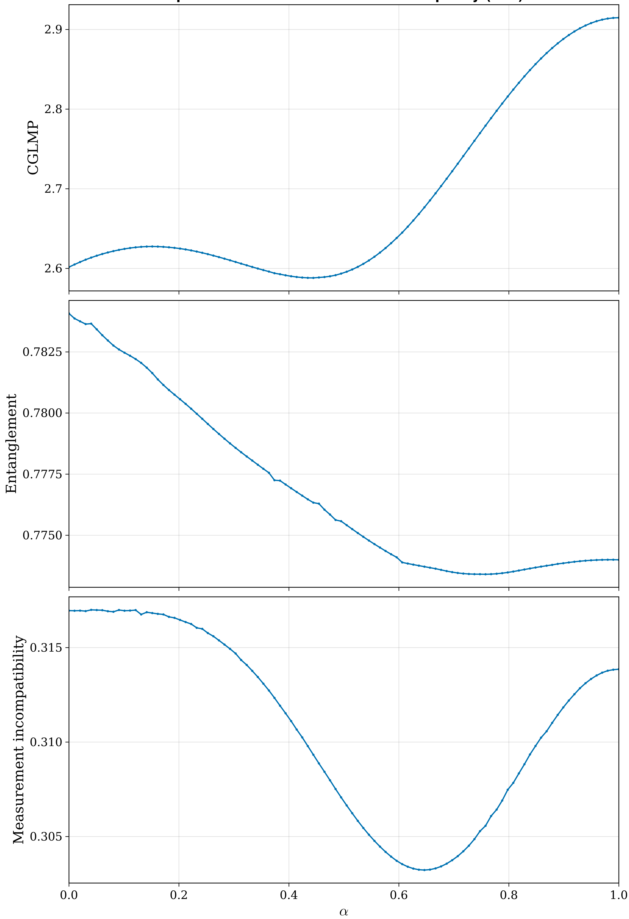
Optimal violation of the CGLMP inequality (d=3)
