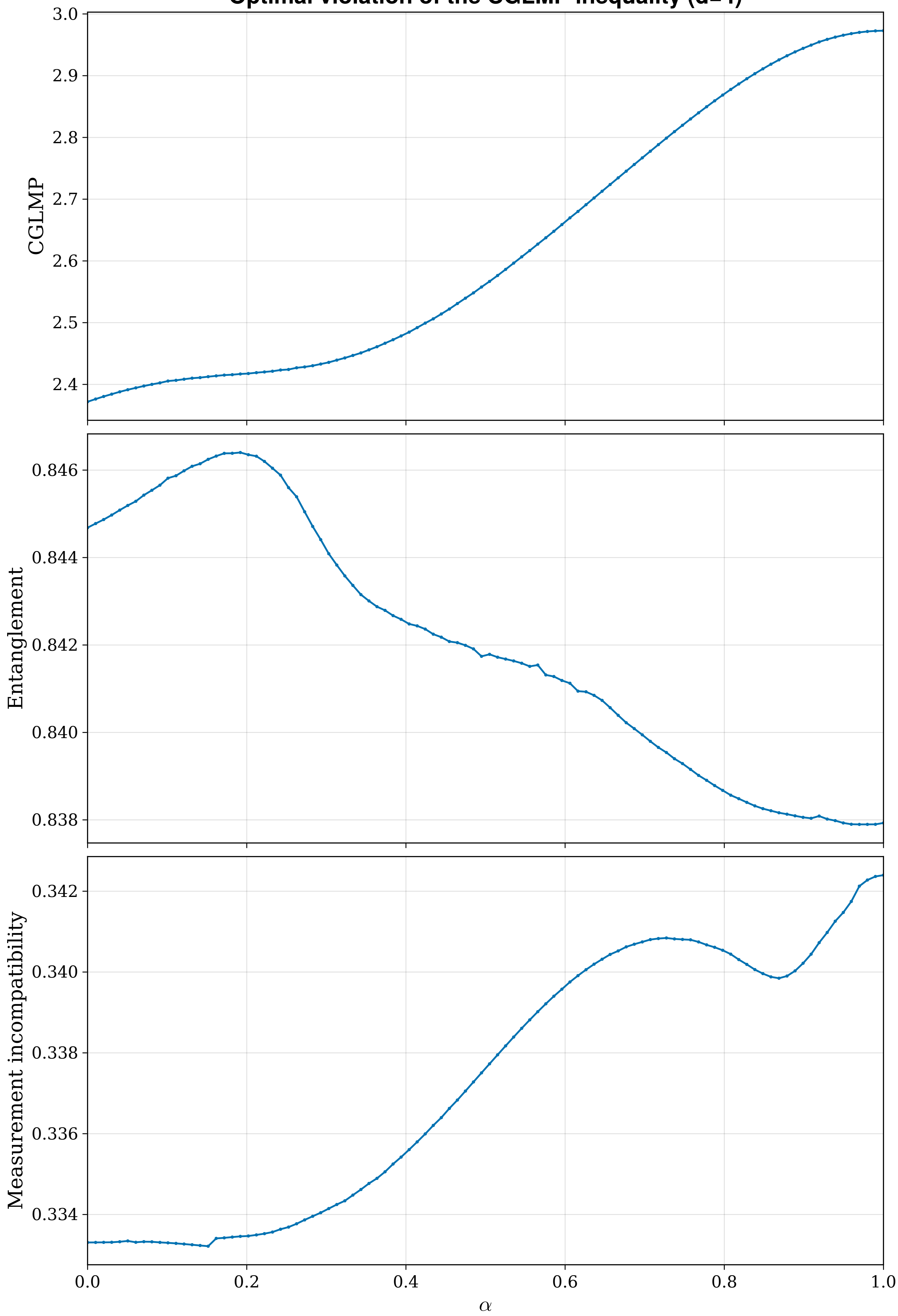
Optimal violation of the CGLMP inequality (d=4)
