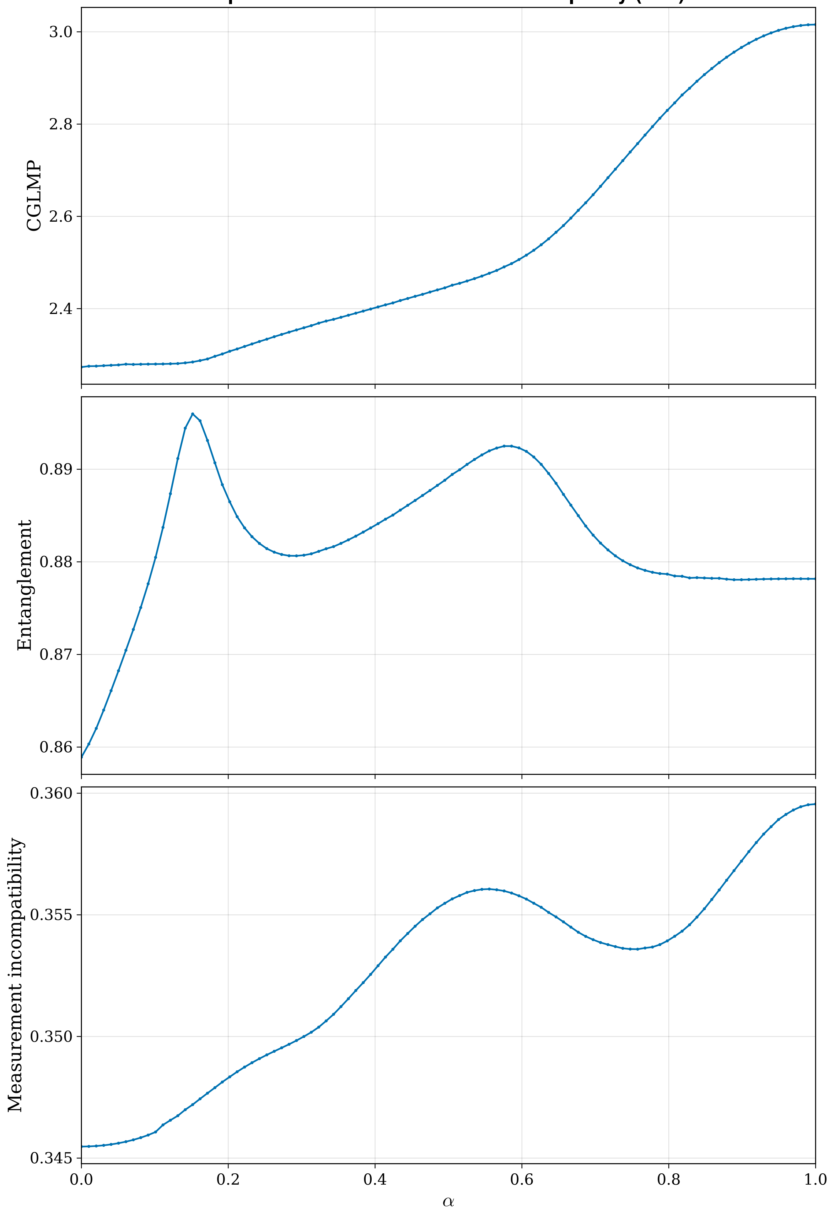
Optimal violation of the CGLMP inequality (d=5)
