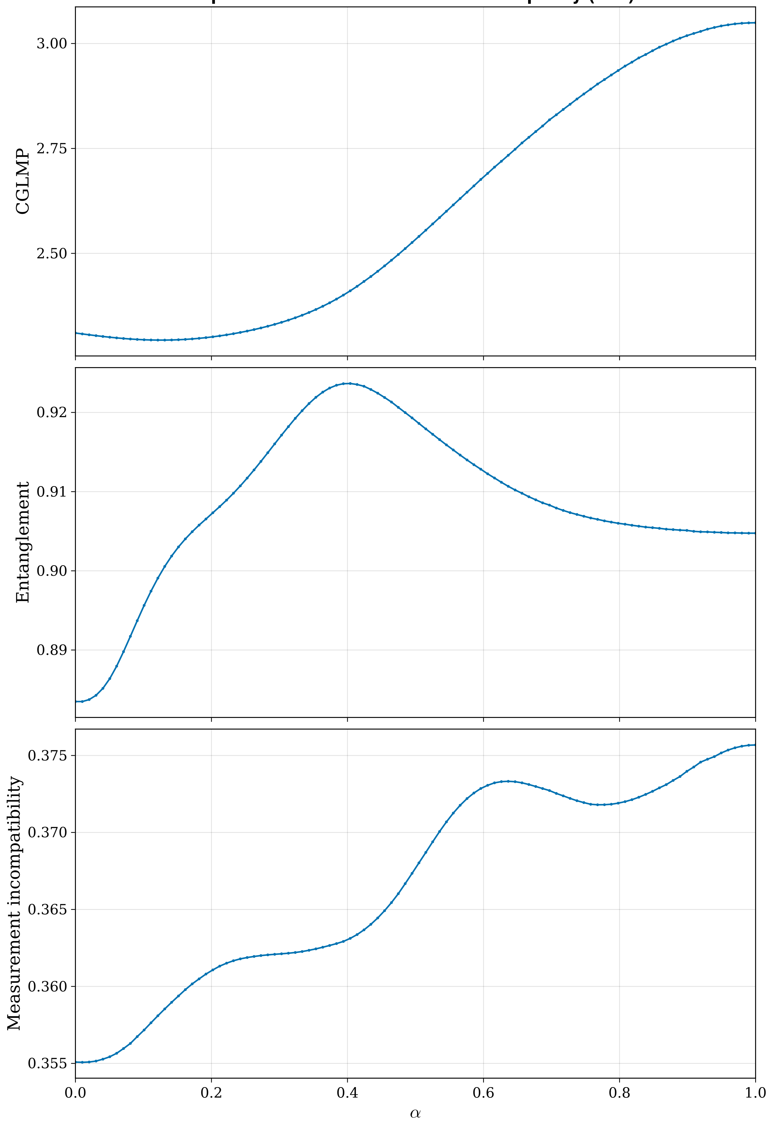
Optimal violation of the CGLMP inequality (d=6)
