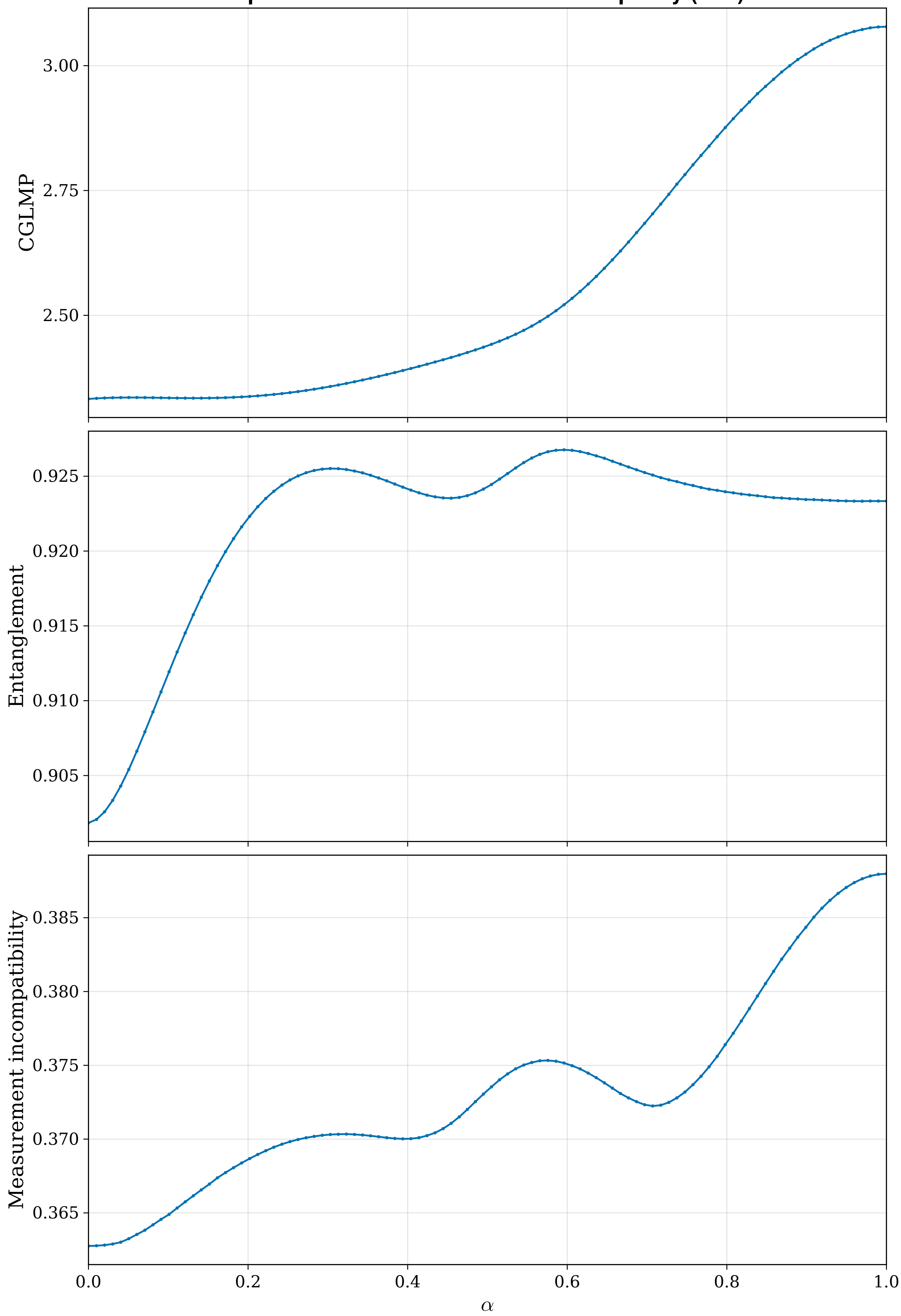
Optimal violation of the CGLMP inequality (d=7)
