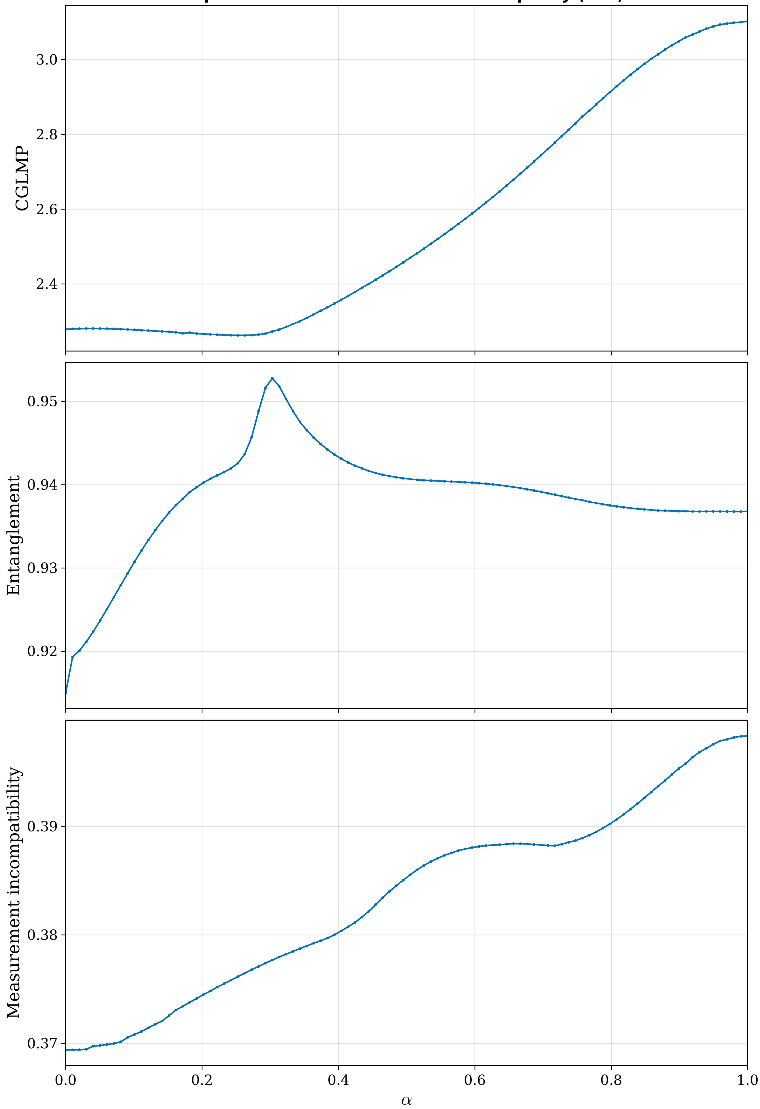
Optimal violation of the CGLMP inequality (d=8)
