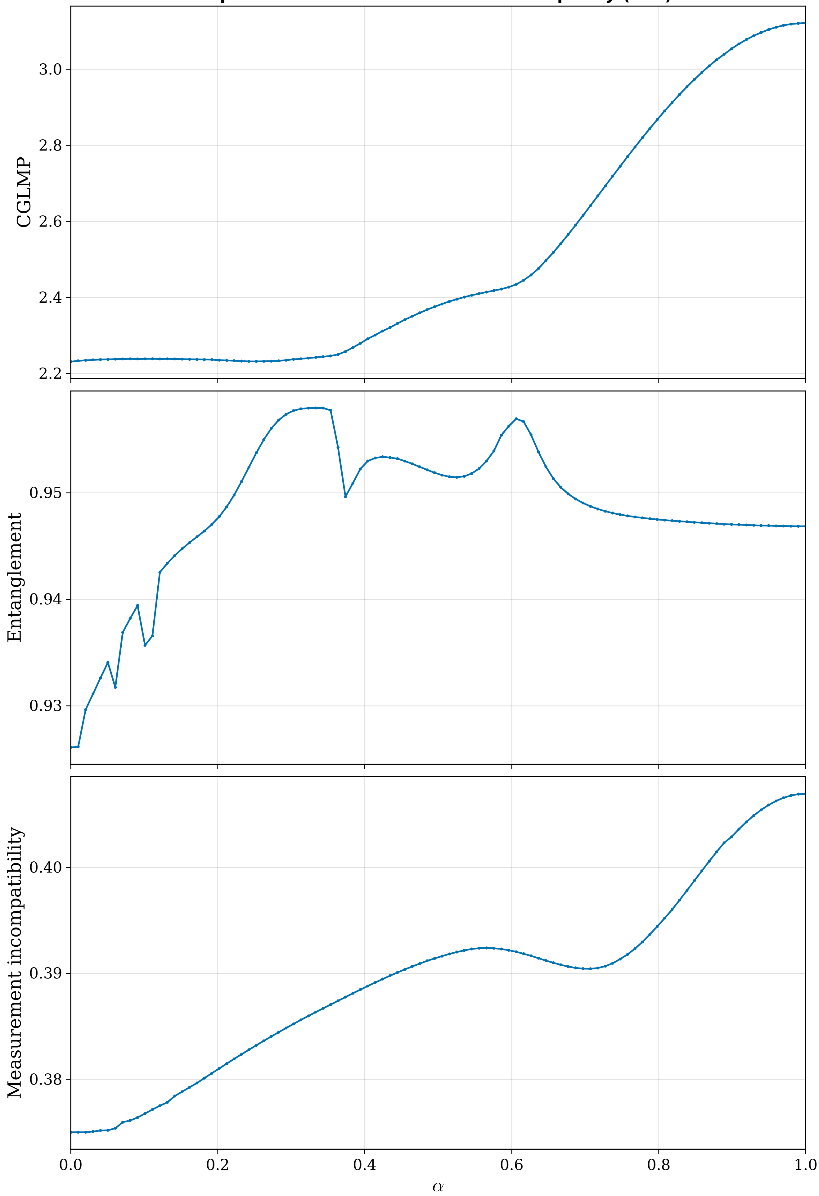
Optimal violation of the CGLMP inequality (d=9)
