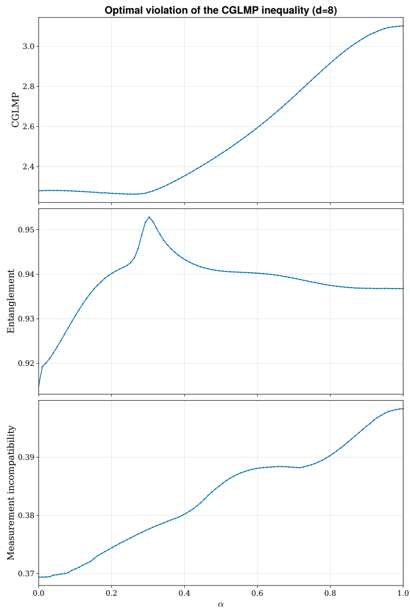
Figure 10. CGLMP inequality violation for d = 8 , and entanglement and measurement incompatibility quantifiers.
