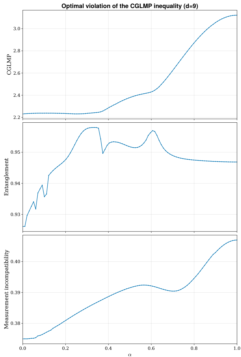
Figure 11. CGLMP inequality violation for d = 9 , and entanglement and measurement incompatibility quantifiers.
