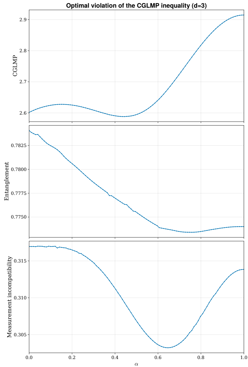
Figure 5. CGLMP inequality violation for d = 3 , and entanglement and measurement incompatibility quantifiers.
