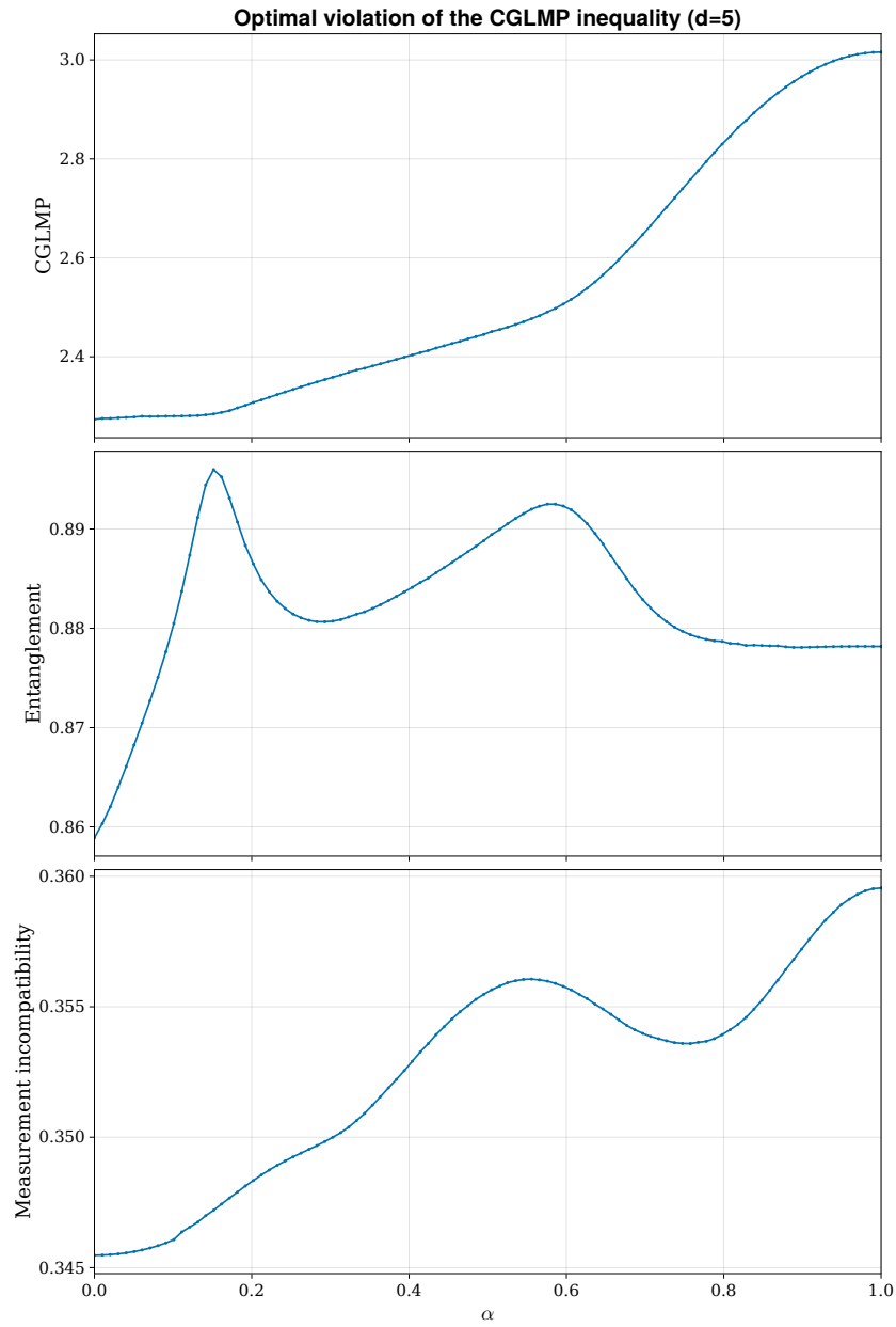
Figure 7. CGLMP inequality violation for d = 5 , and entanglement and measurement incompatibility quantifiers.
