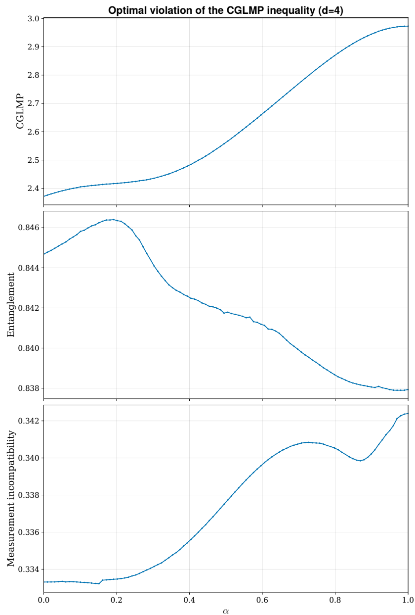
Figure 6. CGLMP inequality violation for d = 4 , and entanglement and measurement incompatibility quantifiers.
