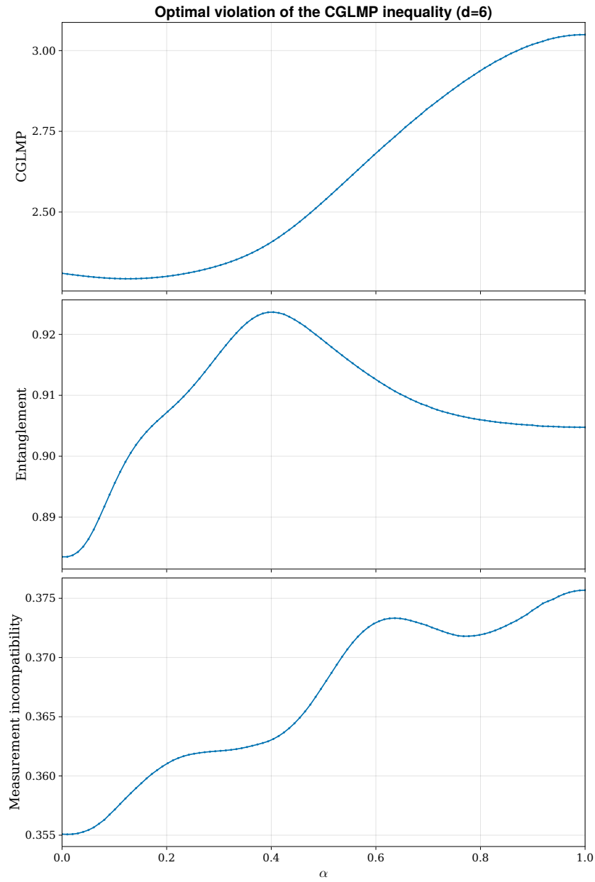
Figure 8. CGLMP inequality violation for d = 6 , and entanglement and measurement incompatibility quantifiers.
