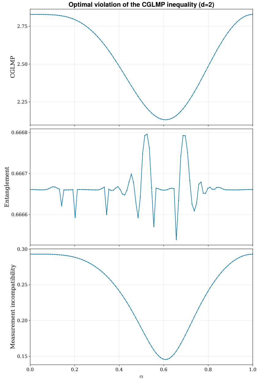
Figure 4. CGLMP inequality violation for d = 2 , and entanglement and measurement incompatibility quantifiers.
