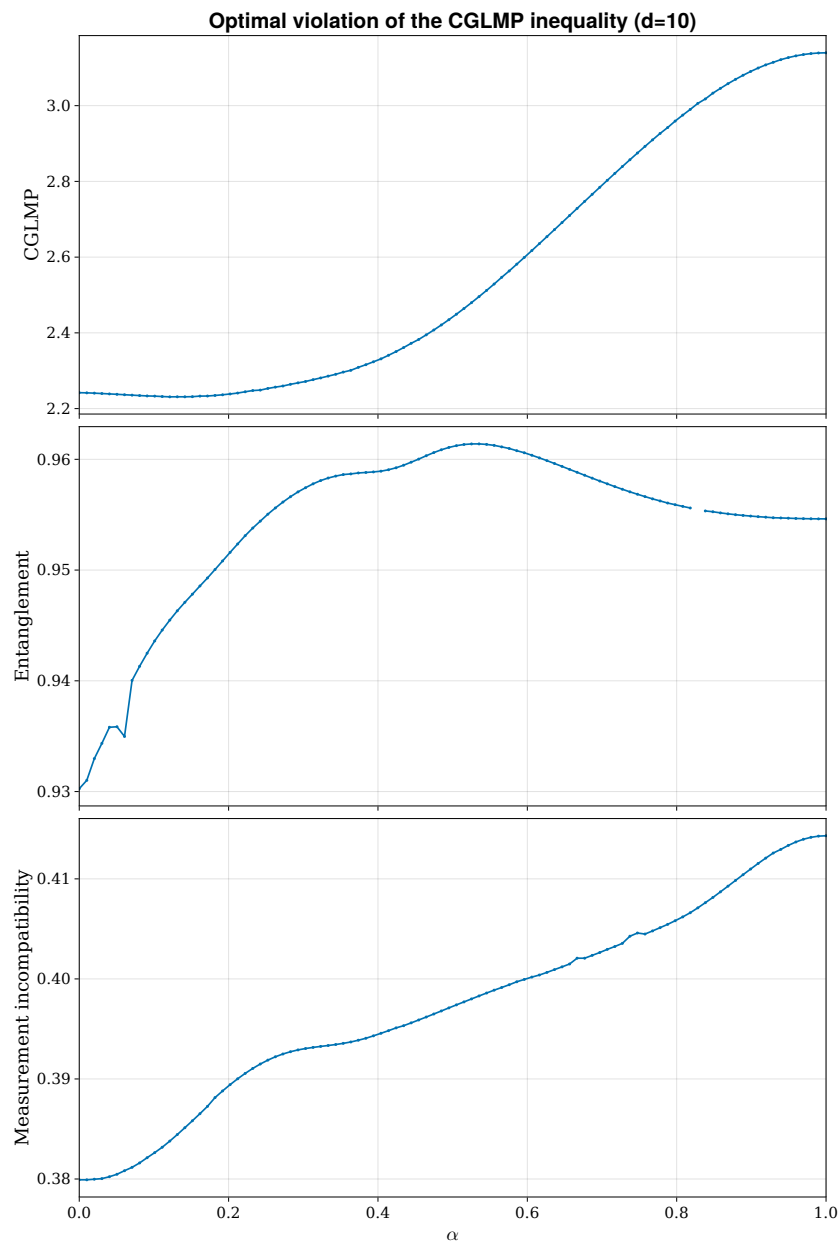
Figure 12. CGLMP inequality violation for d = 10 , and entanglement and measurement incompatibility quantifiers.
