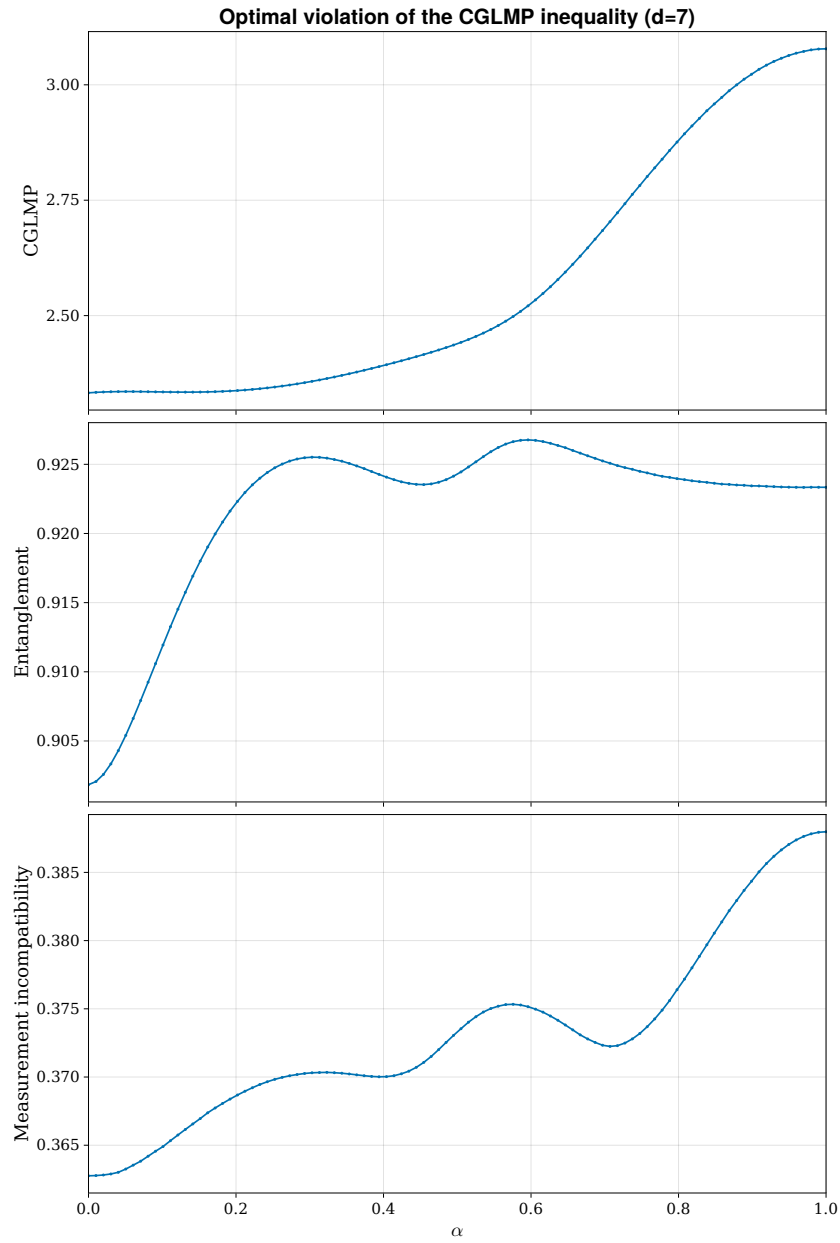
Figure 9. CGLMP inequality violation for d = 7 , and entanglement and measurement incompatibility quantifiers.
