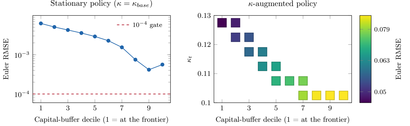
FIGURE 12.—Solution accuracy across the state space
