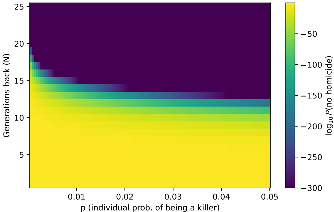
Sensitivity of P to (p, N)
