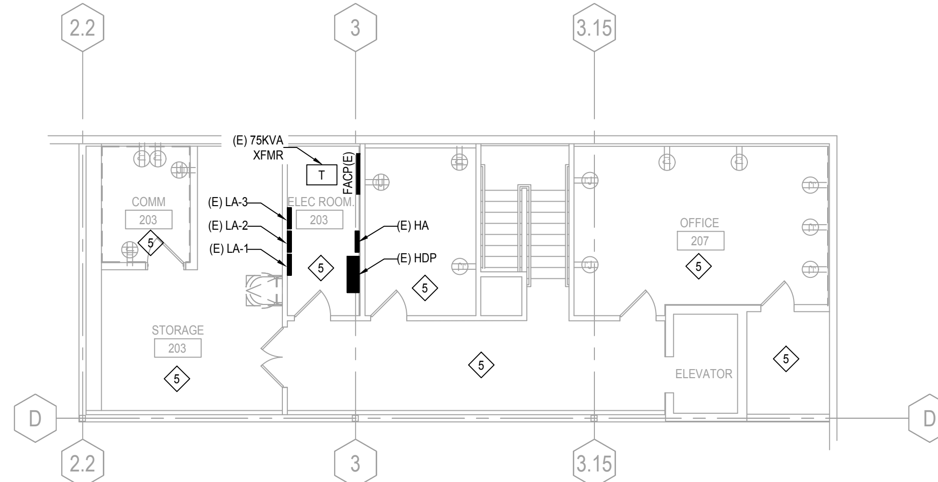
2 PARTIAL SECOND FLOOR PLAN - EXISTING - POWER SCALE: 1/8" = 1'-0"
