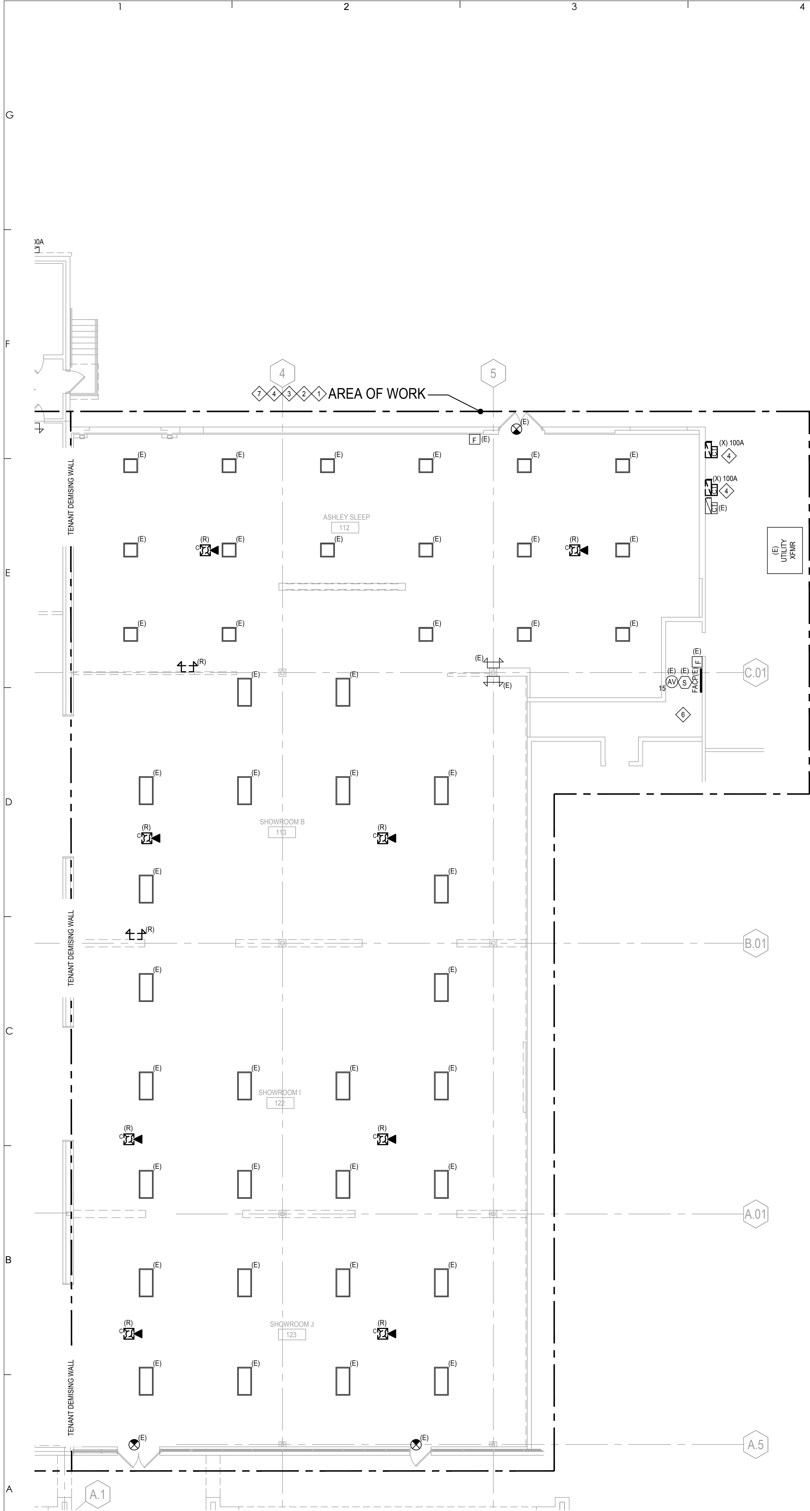
1 PARTIAL FIRST FLOOR PLAN - DEMOLITION SCALE: 1/8" = 1'-0"
