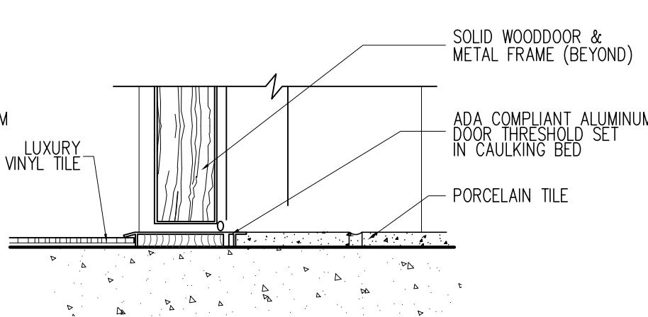
S3 Sill Detail Scale 3"=1'-0"
