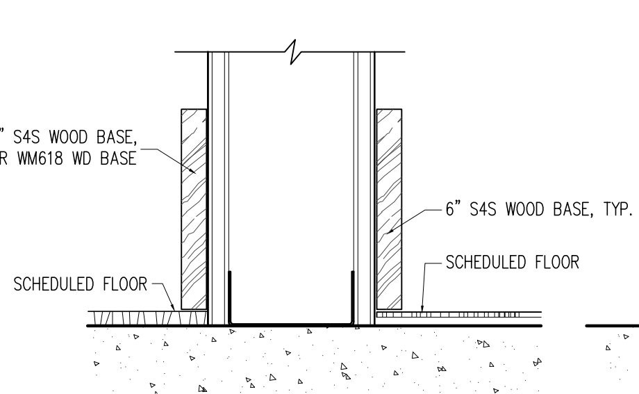
B2 Base Detail Scale 3"=1'-0"
