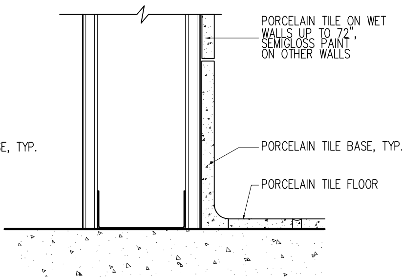
B3 Base Detail Scale 3"=1'-0"
