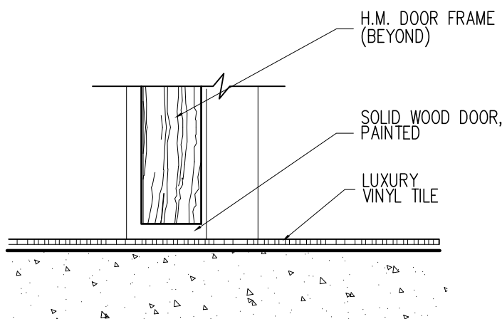
S1 Sill Detail Scale 3"=1'-0"
