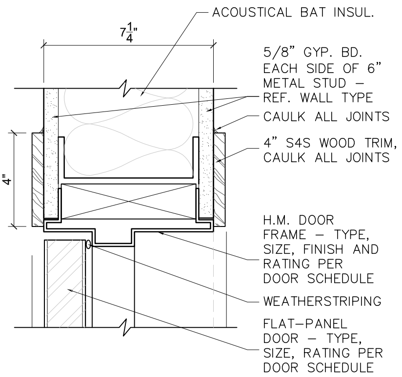
H1/J1 Head/Jamb Detail-Steel Scale 3"=1'-0"
