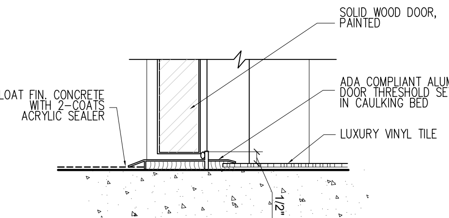
S2 Sill Detail Scale 3"=1'-0"
