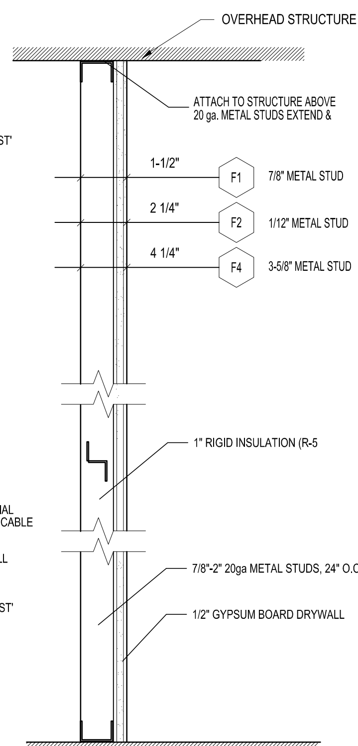
PARTITION TYPE F
