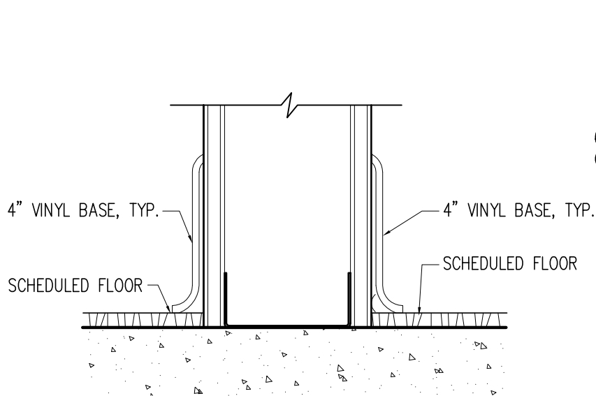
B1 Base Detail Scale 3"=1'-0"
