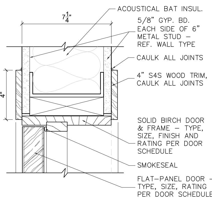
H2/J2 Head/Jamb Detail-Unit Entry Scale 3/4"=1'-0"
