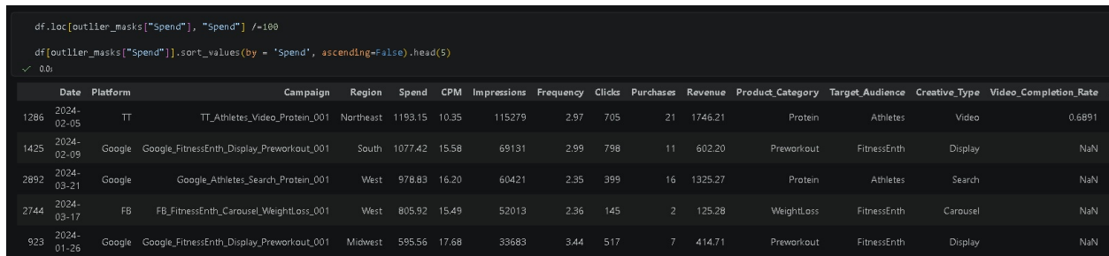
Figure A.12: Datapoints with severe Spend outliers
