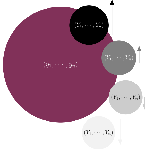
Figure 2: Visualization of the prismatic value of a fixed set of generations, (y_1, \dots, y_n) . Here (Y_1, \dots, Y_n) \sim \pi_\theta(\cdot | x) are sets of generations being sampled and the arrows indicate the value of f(x, Y_{1:n}) . In this visualization, larger intersection between y_{1:n} and the sampled Y_{1:n} tends to correlate with higher scores under the objective f . As such, the prismatic value of y_{1:n} is positive.
