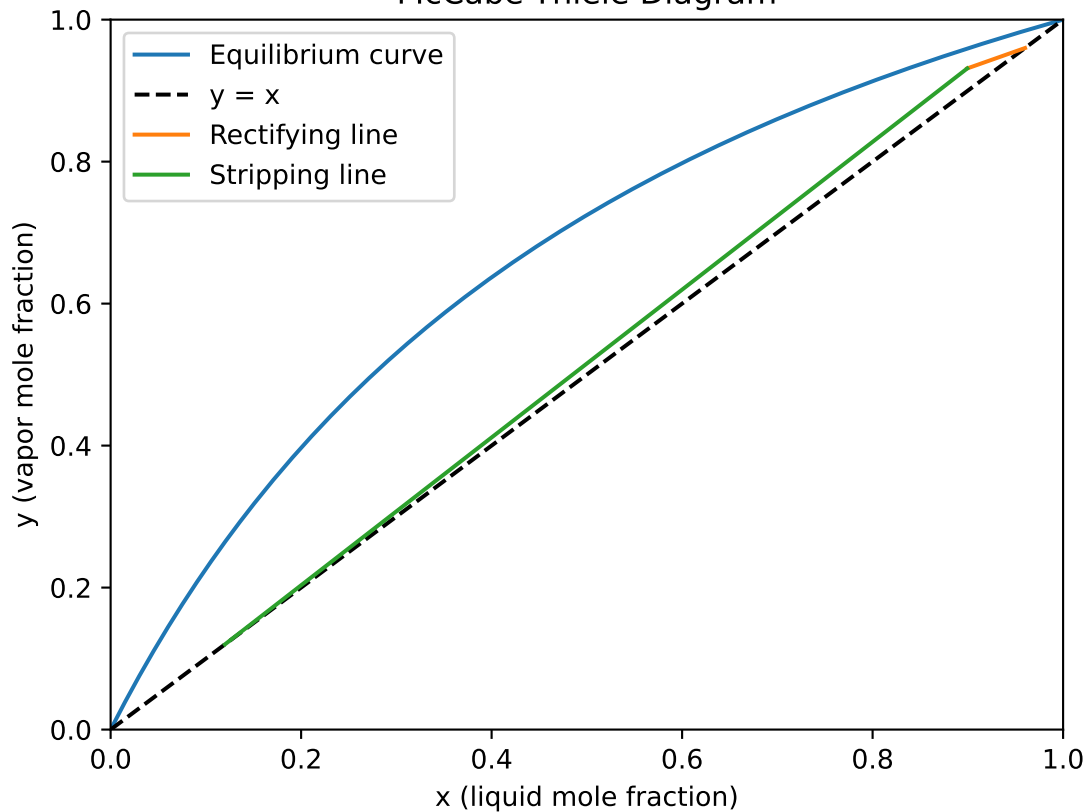
McCabe-Thiele Diagram
