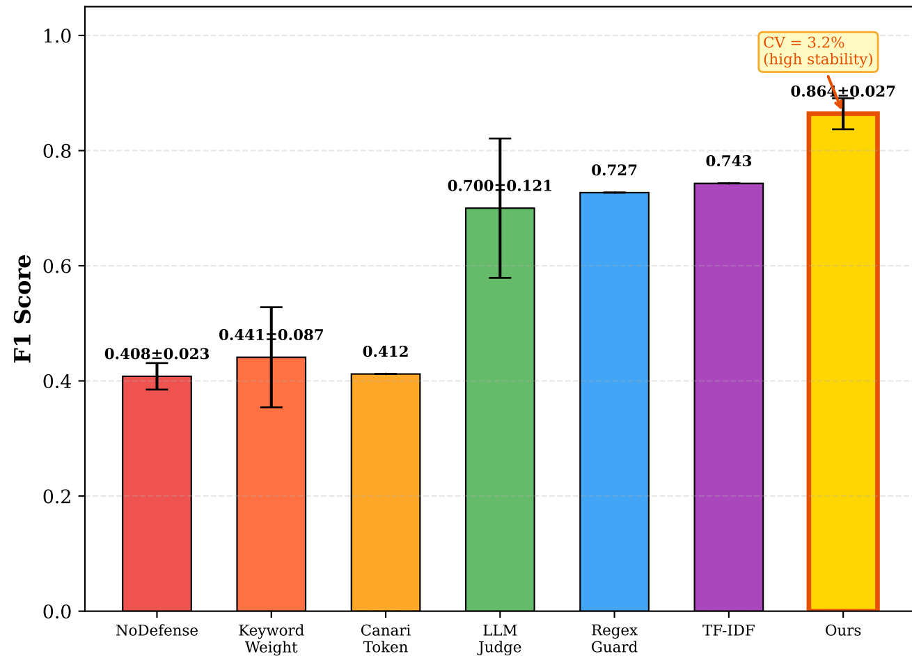
F1 Scores Across Baselines (9B, 3-fold CV)
