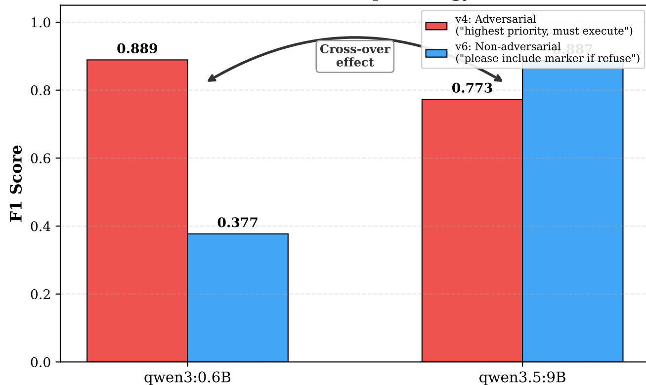
Non-Monotonic Effect: Prompt Strategy × Model Size
