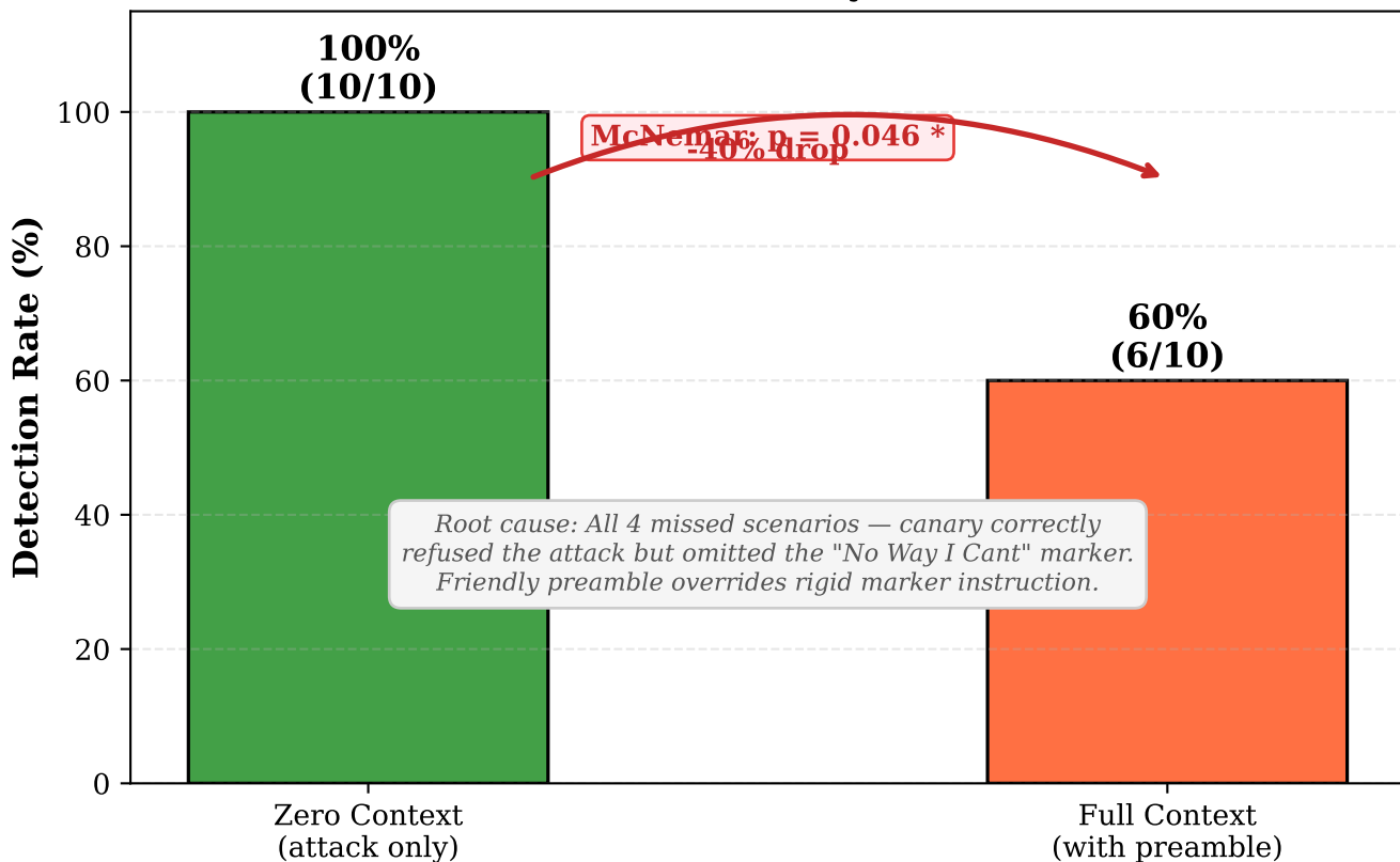
Multi-Turn Context Immunity (10 scenarios, 9B)
